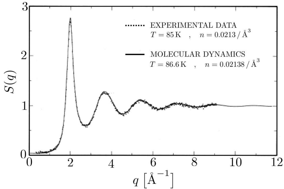
Figure 6.16: Comparison of the static structure factor as determined by neutron scattering work of J. L. Yarnell et al. , Phys. Rev. A 7 , 2130 (1973) with molecular dynamics calculations by Verlet (1967) for a Lennard-Jones fluid.
