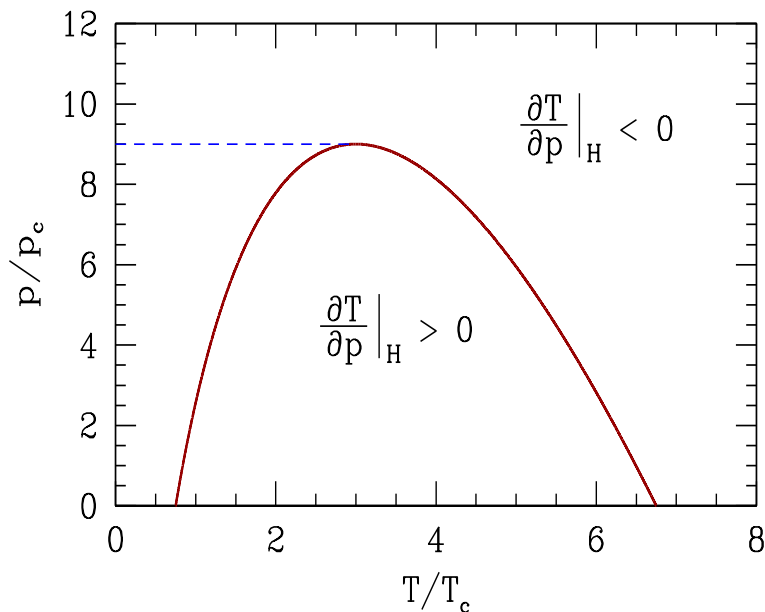
Figure 2.19: Inversion temperature T^*(p) for the van der Waals gas. Pressure and temperature are given in terms of p_c = a/27b^2 and T_c = 8a/27bR , respectively.
