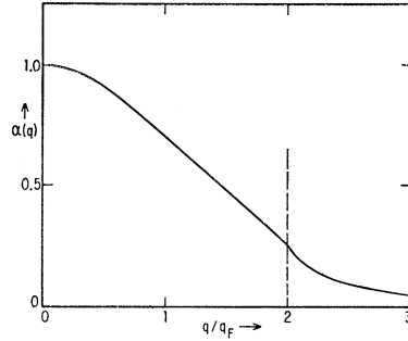
FIG. 1. Behavior of the electronic polarizability \alpha(q) , as function of q (electronic density = 4 \times 10^{23} \text{ cm}^{-3} ).
