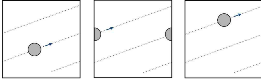
Figure 3.7: Constant phase space velocity at an irrational angle over a toroidal phase space is ergodic, but not mixing. A circle remains a circle, and a blob remains a blob.
