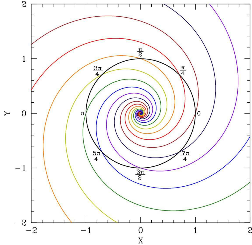
Figure 15.7: Isochrones of the complex amplitude equation \dot{A} = (1 + i\alpha)A - (1 + i\beta)|A|^2A , where A = X + iY .
