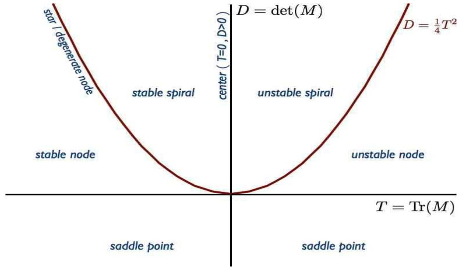
Figure 14.5: Complete classification of fixed points for the N = 2 system.
