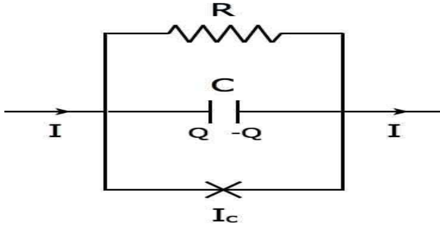
Figure 14.3: . The resistively and capacitively shunted Josephson junction. The Josephson junction is the X element at the bottom of the figure.
