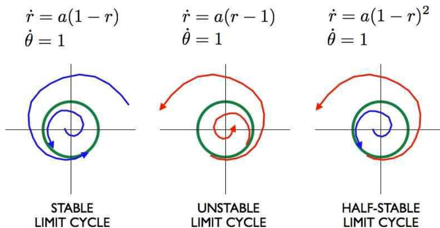
Figure 14.8: Stable, unstable, and half-stable limit cycles.
