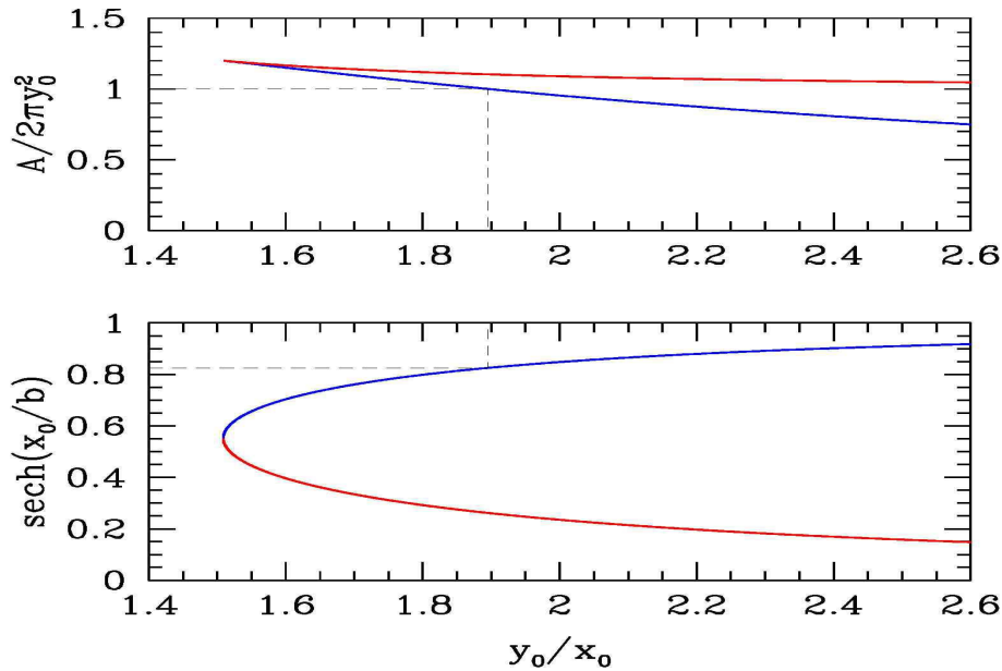
Figure 4.4: Minimal surface solution, with y(x) = b \cosh(x/b) and y(x_0) = y_0 . Top panel: A/2\pi y_0^2 vs. y_0/x_0 . Bottom panel: \text{sech}(x_0/b) vs. y_0/x_0 . The blue curve corresponds to a global minimum of A[y(x)] , and the red curve to a local minimum or saddle point.
