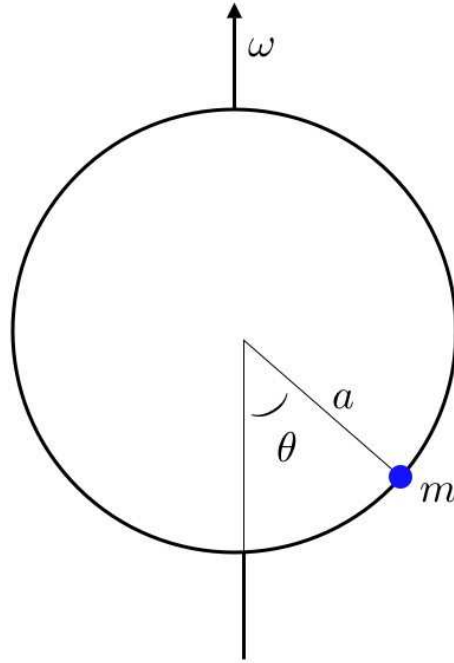
Figure 4.11: A bead of mass m on a rotating hoop of radius a .
