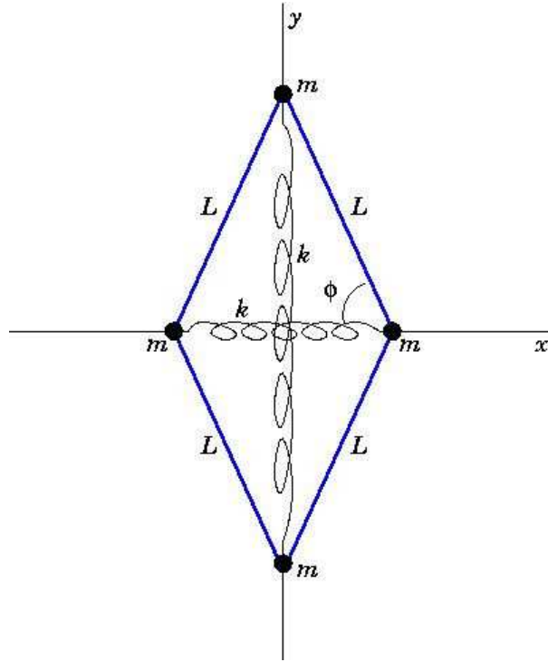
Figure 4.10: The thingy: a rhombus with opening angles 2\phi and \pi - 2\phi .
