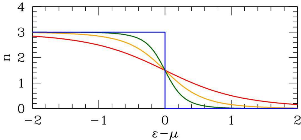
Figure 1: labelpara k = 3 parafermion occupation number versus \varepsilon - \mu for k_B T = 0 , k_B T = 0.25 , k_B T = 0.5 , and k_B T = 1 .
