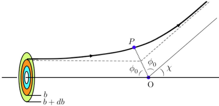
Figure 5.6: Scattering in the CM frame. O is the force center and P is the point of periaapsis. The impact parameter is b , and \chi is the scattering angle. \phi_0 is the angle through which the relative coordinate moves between periaapsis and infinity.
