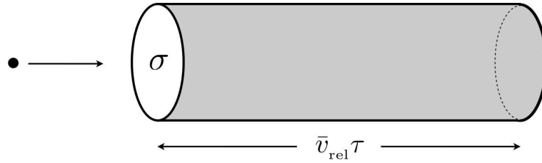
Figure 5.3: Graphic representation of the equation n \sigma \bar{v}_{rel} \tau = 1 , which yields the scattering time \tau in terms of the number density n , average particle pair relative velocity \bar{v}_{rel} , and two-particle total scattering cross section \sigma . The equation says that on average there must be one particle within the tube.
