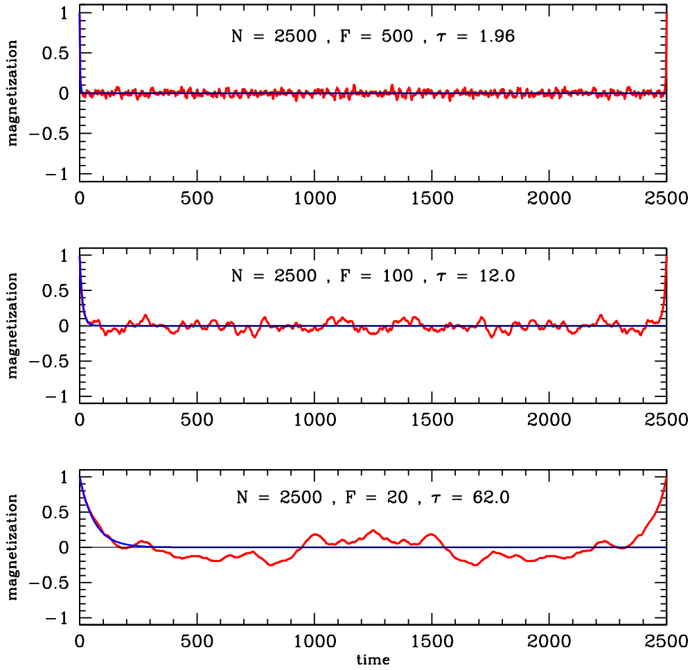
Figure 5.5: Three simulations of the Kac ring model with N = 2500 sites and three different concentrations of flippers. The red line shows the magnetization as a function of time, starting from an initial configuration in which 100% of the spins are up. The blue line shows the prediction of the Stosszahlansatz , which yields an exponentially decaying magnetization with time constant \tau .
