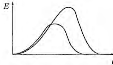
Fig. 2.19. Electric field within a stationary moving domain in AsGa. The domains are moving to the left with the speed 1.2 \times 10^7 \text{ cm s}^{-1} .
