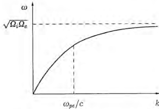
Fig. 5.7. Magneto-sound dispersion in the case of transverse propagation.
