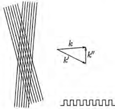
Fig. 2.14. A moire as the result of a nonlinear superposition of two plane waves.
