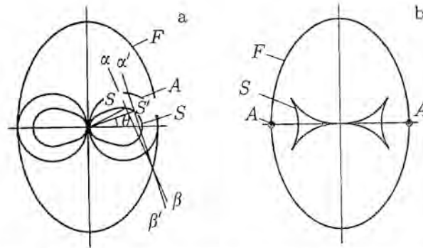
Fig. 5.3. Phase (a) and group (b) diagrams: A — the Alfvén wave, S and F — slow and fast magneto-acoustic waves.
