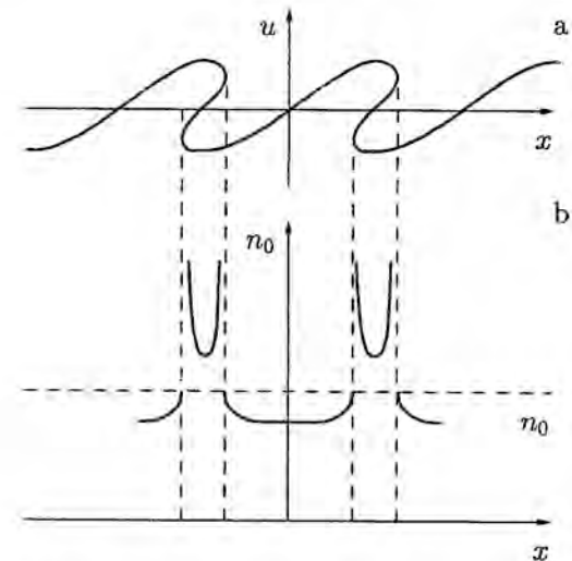
Fig. 2.2. Multibeam pattern as a result of modulated beam evolution. The beam velocity (a) and density (b) are shown.
