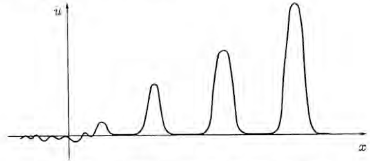
Fig. 2.5. Soliton from an initial pulsed perturbation with \sigma = 8 . According to calculations by Yu. Berezin and V. Karpman [1].
