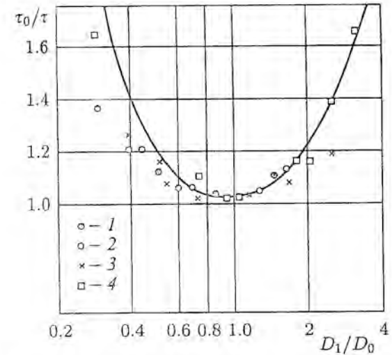
Fig. 4.6. Dependence of the lifetime of a decaying plasma in a toroidal tube upon the diffusion coefficient [Helium, R = 28 cm, a = 0.3 cm, pressure (in mm of mercury): 1 — 0.025, 2 — 0.040, 3 — 0.055, 4 — 0.120].
