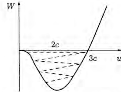
Fig. 2.8. Particle motion in a potential well W(u) in the presence of dissipation.
