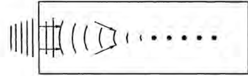
Fig. 2.12. Optical self-focusing.
