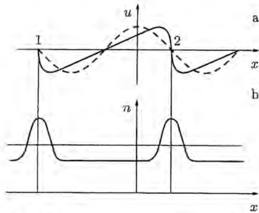
Fig. 2.1. Wave turnover in the case of a beam of noninteracting particles. Evolution of the beam velocity (a) and density (b).
