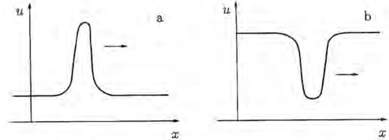
Fig. 2.4. Solitons in a medium with a weak negative (a) and positive (b) dispersion.
