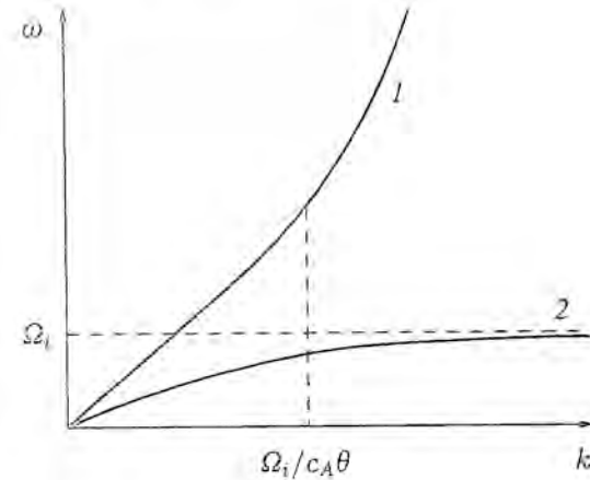
Fig. 5.8. Magneto-sound 1 and Alfvén wave 2 dispersion in the case of oblique propagation.
