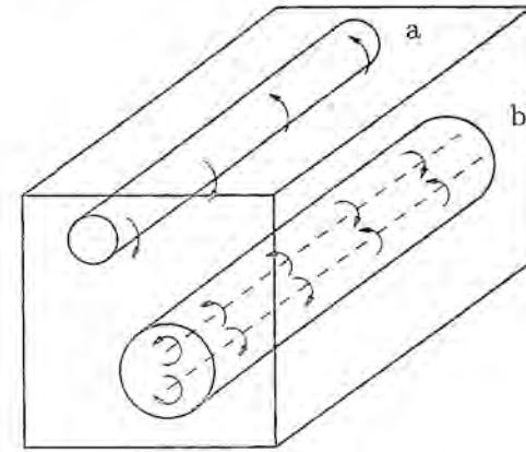
Fig. 5.2. Plasma displacements in Alfvén waves.
