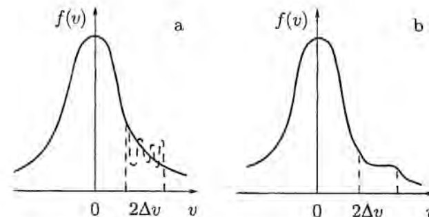
Fig. 3.2. Formation of small-scale oscillations (a) and of a "plateau" (b) on the distribution function profile.
