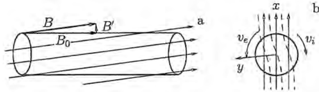
Fig. 4.3. Plasma rotation in a tilted magnetic field.
