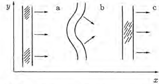
Fig. 2.11. Soliton oscillations in the case of weak negative dispersion.
