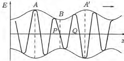
Fig. 2.13. Wave packet selfcompression — envelope instability.
