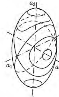
Fig. 2.16. Trajectories of three interacting waves.
