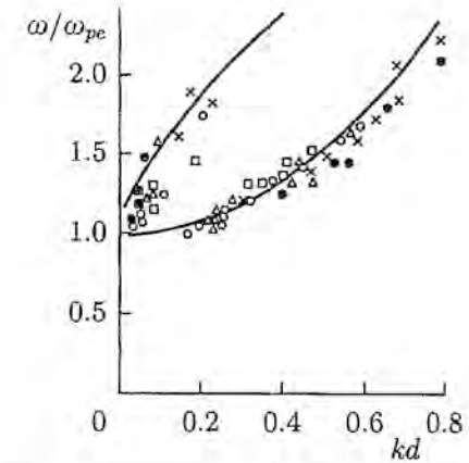
Fig. 3.6. Dispersion curves for Langmuir waves.
