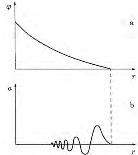
Fig. 1.6. Phase (a) and amplitude (b) dependence upon the distance from a localized pulsed ion sound source.
