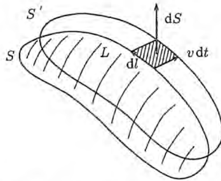
Fig. 4.1. Motion of a contour in a plasma.
