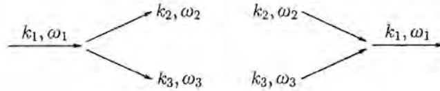
Fig. 2.15. Three-wave processes.
