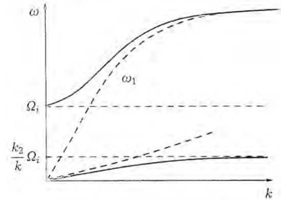
Fig. 5.6. Ion-sound dispersion.
