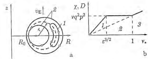
Fig. 4.5. (a) Trajectories of trapped 1 and transitory 2 particles. (b) Dependence of the transport coefficients on the dimensionless collision frequency v_* = \nu q R / v_T .
