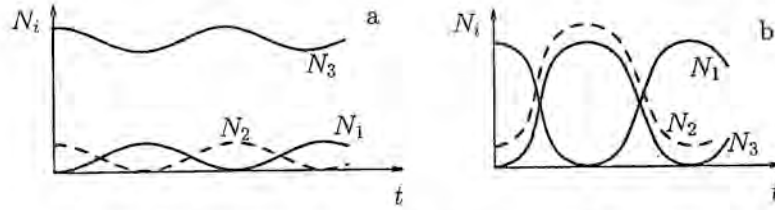
Fig. 2.17. Dependence of amplitudes of three interacting waves upon time in the case of stable (a) and unstable (b) initial states.
