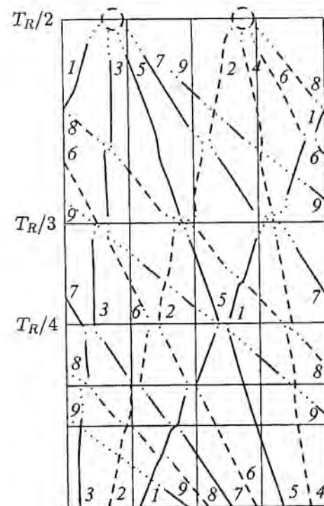
Fig. 2.7. Soliton trajectories. T_R is the time of return to the initial state.
