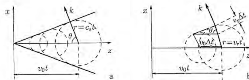
Fig. 1.4. Wave superposition produced by a moving body in the cases of nondispersive (a) and dispersive (b) media.
