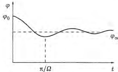
Fig. 3.4. Temporal evolution of a wave of a finite amplitude.
