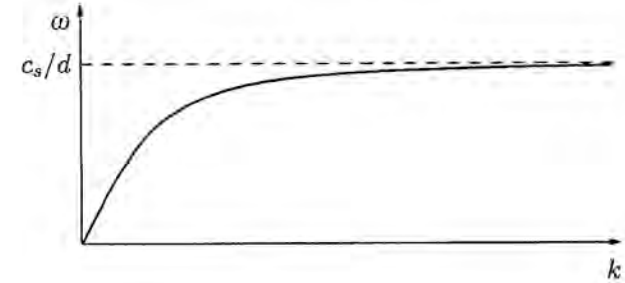
Fig. 1.1. Dependence of the ion wave frequency on the wave number.
