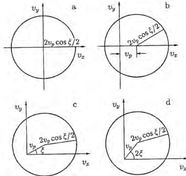
Fig. 3.13. Distribution of velocities of the electrons. (a) — for a three-pulse echo before the third pulse; (b) — just after the third pulse; (c) — at the instant of the first echo; (d) — at the instant of the second echo.
