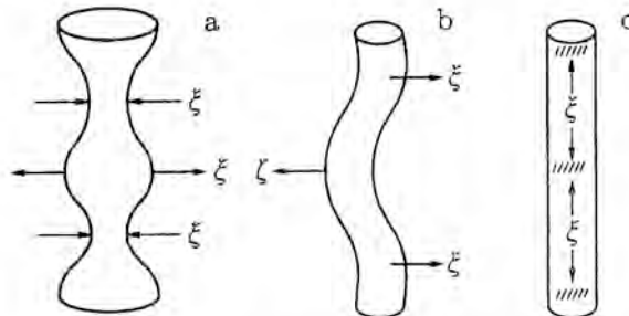
Fig. 5.1. Plasma displacements corresponding to magneto-sound (a), Alfvén (b) and ion-sound (c) oscillations.
