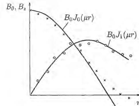
Fig. 4.2. Magnetic field components inside a diffusive pinch.
