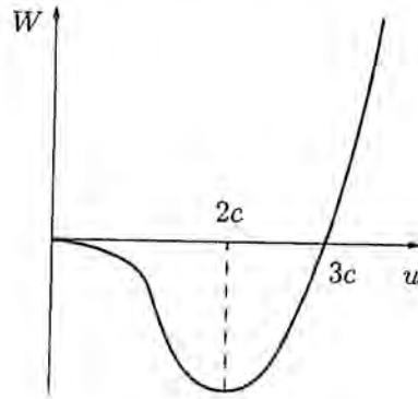
Fig. 2.3. "Potential energy" for a periodic wave.
