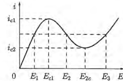
Fig. 2.20. Dependence of the current on the applied voltage for a semiconductor with a negative differential conductance.
