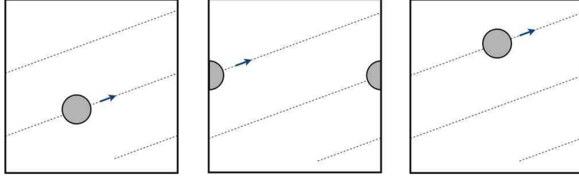
Figure 5.7: Constant phase space velocity at an irrational angle over a toroidal phase space is ergodic, but not mixing. A circle remains a circle, and a blob remains a blob.
