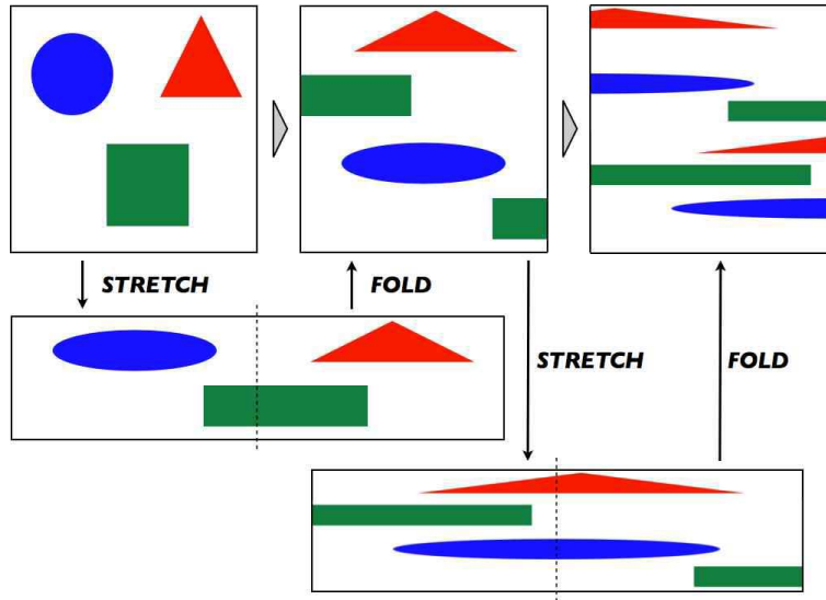
Figure 5.8: The baker's transformation is a successive stretching, cutting, and restacking.
