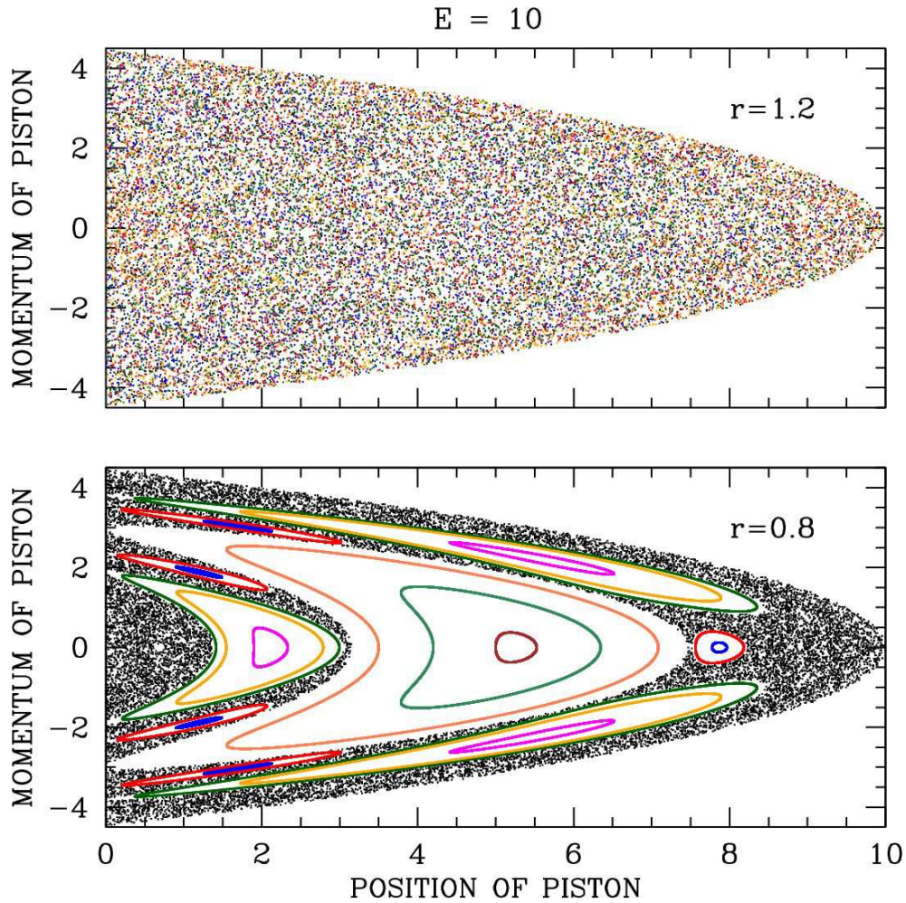
Figure 5.12: Poincaré sections for the ball and piston head problem. Each color corresponds to a different initial condition. When the mass ratio r = m/M exceeds unity, the system apparently becomes ergodic.
