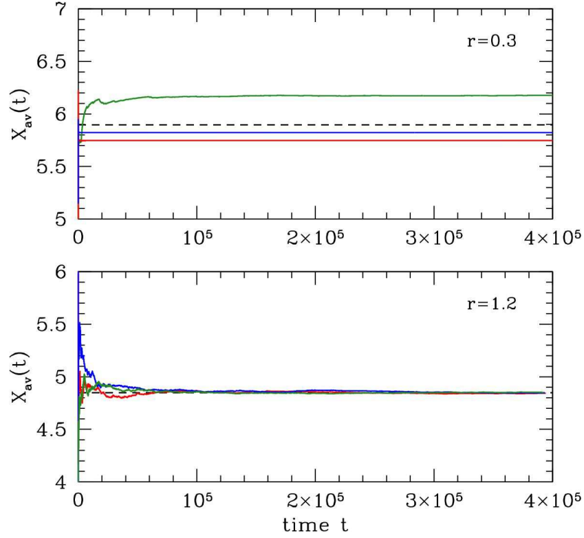
Figure 5.13: Long time running numerical averages X_{\text{av}}(t) \equiv t^{-1} \int_0^t dt' X(t') for r = 0.3 (top) and r = 1.2 (bottom), each for three different initial conditions, with E = 10 in all cases. Note how in the r = 0.3 case the long time average is dependent on the initial condition, while the r = 1.2 case is ergodic and hence independent of initial conditions. The dashed black line shows the restricted microcanonical average, \langle X \rangle_{\mu ce} = \frac{(2+r)}{(1+r)} \cdot \frac{1}{3} E .
