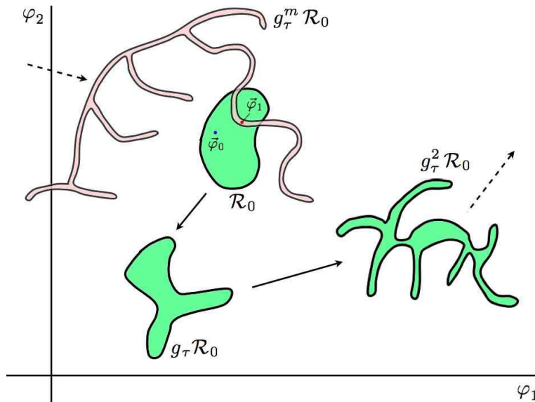
Figure 5.2: Successive images of a set \mathcal{R}_0 under the \tau -advance mapping g_\tau , projected onto a two-dimensional phase plane. The Poincaré recurrence theorem guarantees that if phase space has finite volume, and g_\tau is invertible and volume preserving, then for any set \mathcal{R}_0 there exists an integer m such that \mathcal{R}_0 \cap g_\tau^m \mathcal{R}_0 \neq \emptyset .
