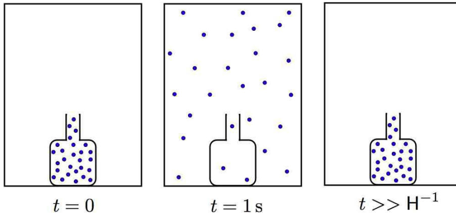
Figure 5.3: Poincaré recurrence guarantees that if we remove the cap from a bottle of perfume in an otherwise evacuated room, all the perfume molecules will eventually return to the bottle! (Here H is the Hubble constant.)
