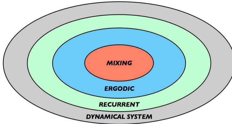
Figure 5.11: The hierarchy of dynamical systems.
