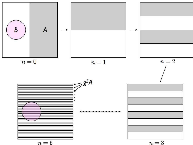
Figure 5.9: The multiply iterated baker’s transformation. The set A covers half the phase space and its area is preserved under the map. Initially, the fraction of B covered by A is zero. After many iterations, the fraction of B covered by g^n A approaches \frac{1}{2} .
