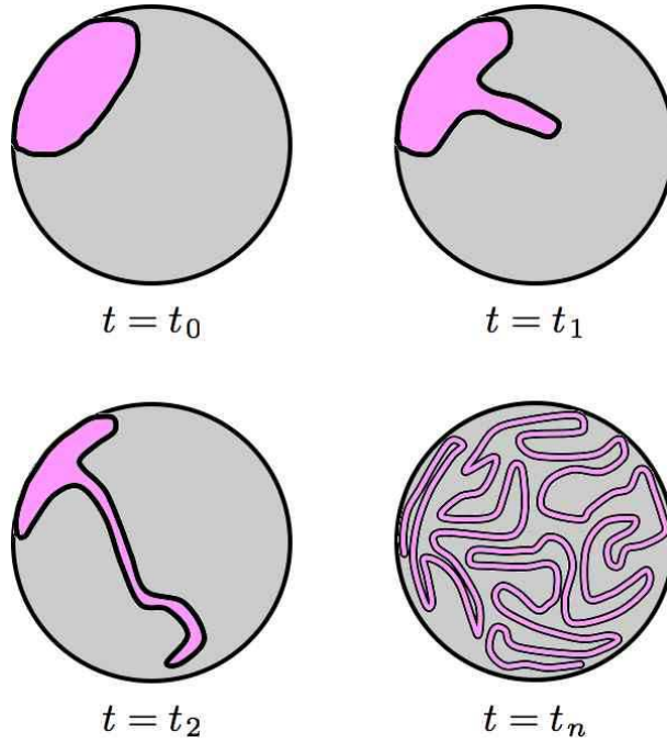
Figure 5.1: Time evolution of two immiscible fluids. The local density remains constant.
