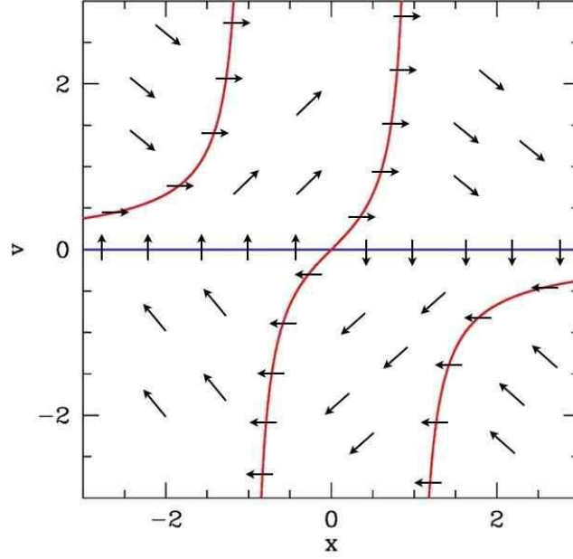
Figure 3.16: Sketch of phase flow and nullclines for the oscillator \ddot{x} + \epsilon(x^4 - 1)\dot{x} + x = 0 . Red nullclines: \dot{v} = 0 ; blue nullcline: \dot{x} = 0 .
