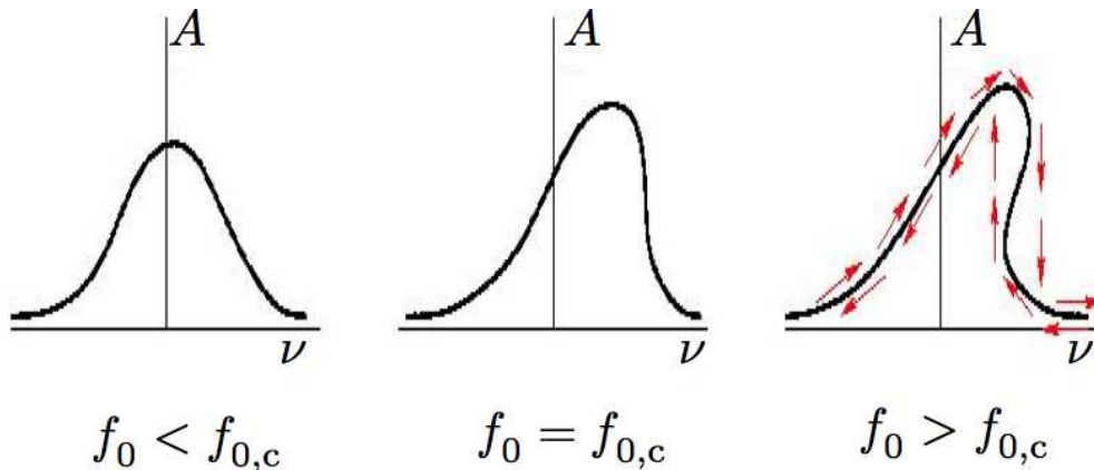
Figure 3.2: Amplitude A versus detuning \nu for the forced Duffing oscillator for three values of the drive f_0 . The critical drive is f_{0,c} = \frac{16}{3^{5/4}}\mu^{3/2} . For f_0 > f_{0,c} , there is hysteresis as a function of the detuning.
