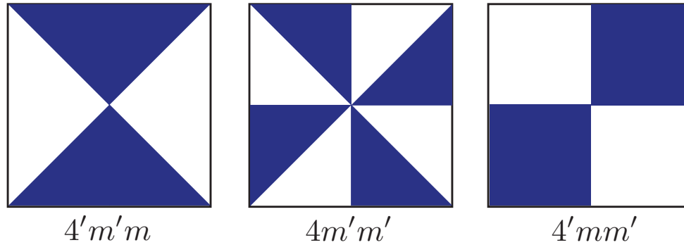
Figure 7.1: Colored squares and their magnetic point group symmetries.
