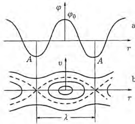
Fig. 3.1. Phase trajectories of electrons in a wave.
