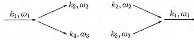
Fig. 2.15. Three-wave processes.
