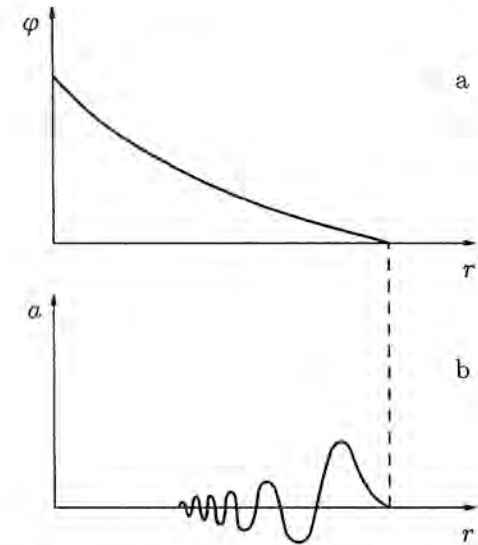
Fig. 1.6. Phase (a) and amplitude (b) dependence upon the distance from a localized pulsed ion sound source.
