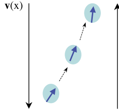
Fig. 5.8. Wave packet (which is denoted by the shade) with wave vector \mathbf{k} (thick solid arrow) moves in the presence of large-scale strain field \mathbf{v}(x) . Thin dotted arrows show motion of a packet in real space.
