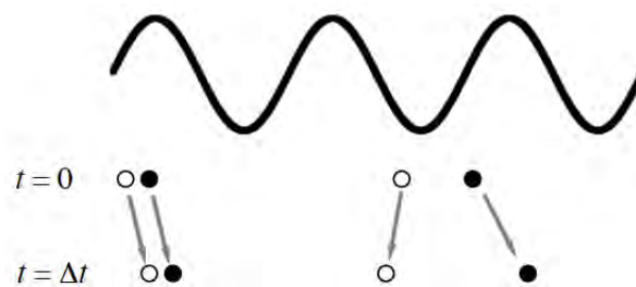
Fig. 8.9. Relative motion of two particles, being scattered by the fluctuations. The growth of separation depends on the initial separation.
