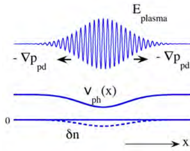
Fig. 7.3. Inhomogeneous plasma waves generate the pressure field for the mean electron dynamics. Density perturbation of the acoustic wave \delta n_e (dotted line) gives rise to the modulation of the refractive index of plasma waves (thick solid line).
