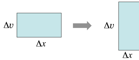
Fig. 8.5. Conservation of a volume of an element in the phase space.
