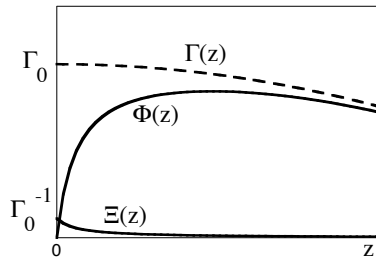
Fig. 6.11. Schematic drawing of the Laplace transforms \Phi(z) , \Gamma(z) and \Xi(z) .
