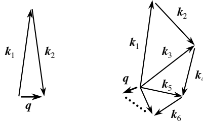
Fig. 7.2. Comparison of disparate scale interaction (left) and inverse cascade (right). The long-wavelength perturbation (characterized by \mathbf{q} ) is directly generated by, e.g., parametric instability in the disparate-scale interactions.
