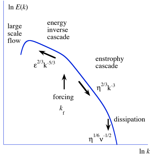
Fig. 2.17. Schematic of energy spectrum for dual cascade.
