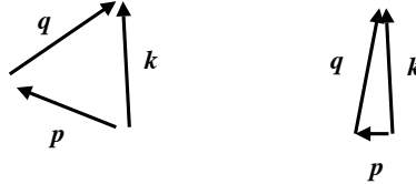
Fig. 6.6. Examples of triad pairs. Interaction among like-scale perturbations (left) and that among disparate scales (right).
