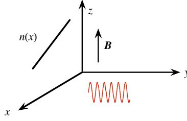
Fig. 6.12. Geometry of inhomogeneous plasma and magnetic field
