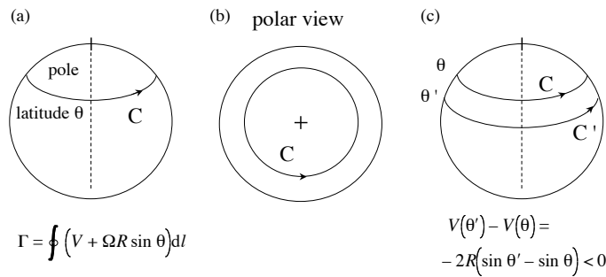
Fig. 8.3. Contour C at latitude \theta and the circulation \Gamma (a). Polar view is illustrated in (b). When the contour is moved to lower latitude, \theta \rightarrow \theta' , conservation of circulation deduces the westward circulation (c).
