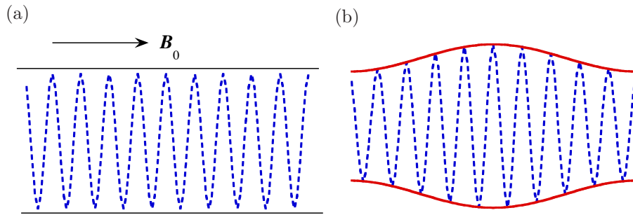
Fig. 9.7. (a) Unperturbed wave train and its envelope. (b) Localized modulational perturbation.
