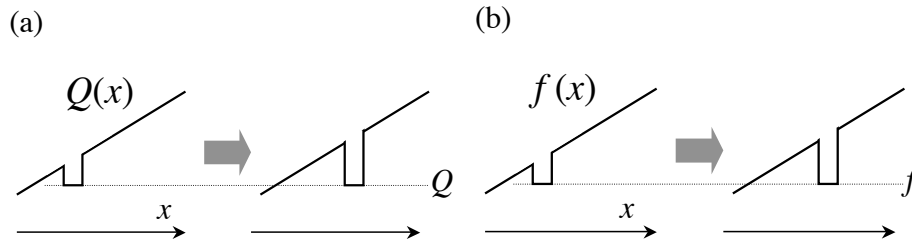
Fig. 8.7. Conservation of the potential vorticity PV in the QG system (a). When a dip moves to a region of higher mean PV, the perturbation grows. Associated with this, the gradient of mean PV relaxes. Conservation of the total number density f in the Vlasov system (b). In this illustration, a dip of f grows by the expense of the relaxation of the mean.
