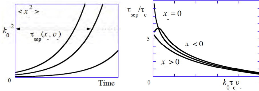
Fig. 8.10. Evolution of statistical average of separation for various initial separations (left). The separation time is \tau_{sep} defined for each initial condition. The separation time is shown as a function of initial separation in velocity space v_- .
