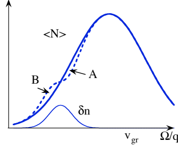
Fig. 7.6. Relaxation of the quasiparticle action density owing to the interaction with acoustic waves (in a one dimensional problem). The density \langle N \rangle is subject to flattening and turns to the one shown by the dashed line. The areas 'A' and 'B' in this figure are equal. However, the frequency of plasma waves is higher in the domain 'A' than that in 'B', so that the energy content in 'A' is larger than that in 'B'. The difference of the energy in 'A' and 'B' is converted into acoustic waves.
