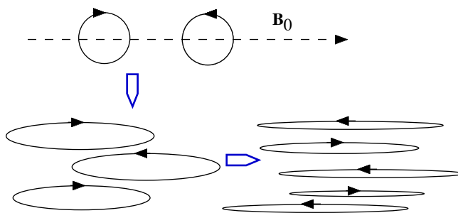
Fig. 9.5. Comparison of the isotropic Kolmogorov cascade with the anisotropic Alfvén turbulence cascade. In the latter case, anisotropy increases as the cascade progresses.
