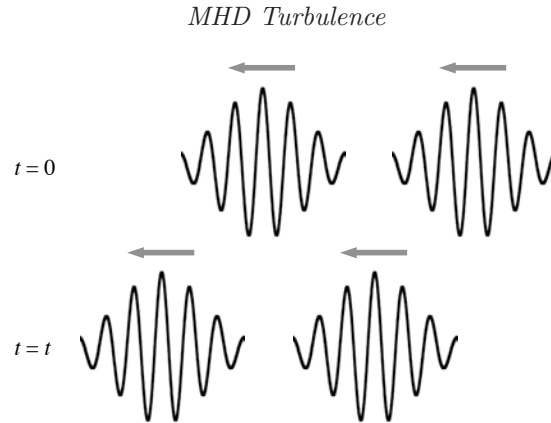
Fig. 9.2. Parallel propagating wave streams do not interact.
