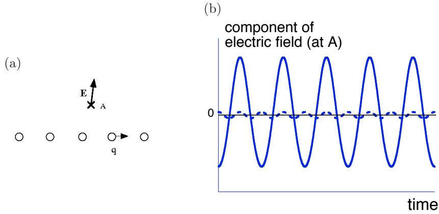
Fig. 2.6. Schematic illustration that the discreteness of particles is the origin of radiations. A train of charged particles (charge q , distance d ) are moving near by the observation point A (a). The vertical component of the electric field observed at point A (b). When each particle is divided into two particles, (i.e., charge per particle is q/2 and distance between particles is d/2 ), the amplitude of observed field becomes smaller (dashed curve in (b)).
