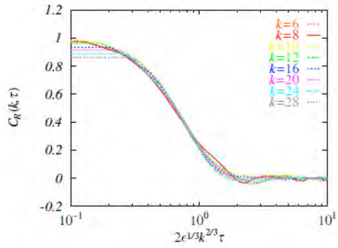
Fig. 6.17. Autocorrelation function of the fluctuating force for various choice of test wave number. Unit of time is normalized to \epsilon^{-1/3}k^{-2/3} . (Gotoh et al., 2002; Gotoh, 2006)
