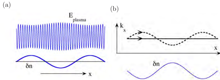
Fig. 7.5. Plasma waves coexist with the acoustic wave (a). The trajectory of quasiparticle of plasma waves in the presence of the acoustic wave (dashed line) and the unperturbed trajectory (solid line), (b). (Schematic drawing.)
