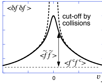
Fig. 8.11. Correlation function \langle \delta f(1)\delta f(2) \rangle as a function of the separation of particle. The collisionless limit (dotted line) and the case where cut-off by collision works at v_- = 0 . Contributions from coherent component and granulations are also noted.
