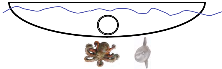
Fig. 6.8. Correlation of observed (Eulerian) signals is affected by sweeping. When a mola mola and an octopus are swept by the sea current, after an elapse of a short time, a fish (observed from a window of a ship) seems to metamorphose into an octopus [After Yoshizawa].
