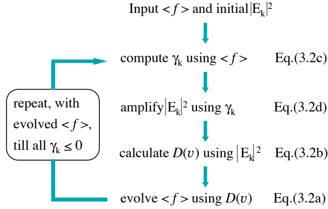
Fig. 3.3. Schematic for implementation of quasilinear theory
