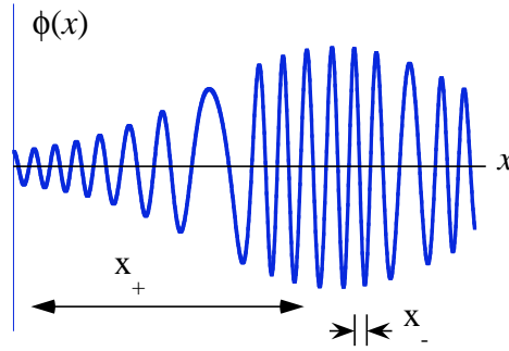
Fig. 3.9. Small scale variable and large scale variable for fluctuations.
