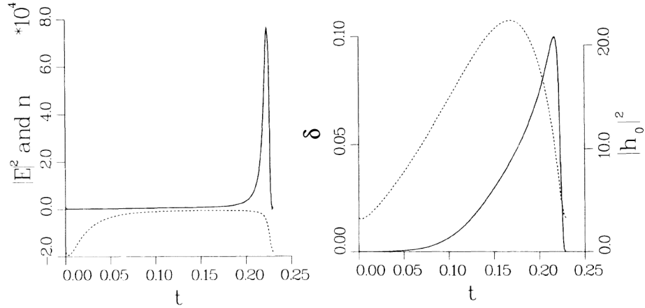
Fig. 7.9. Example of spherical collapse of Langmuir waves. Intensity of waves |E|^2 and perturbation density (dashed line) at the center r = 0 are given in (a). (Parameters are: pump wave intensity |E_0| = 5 , m_i/m_e = 2000 . Normalization units for time, length, electric field and perturbed number density are (3m_i/2m_e)\omega_{pe}^{-1} , (3/2)\sqrt{m_i/m_e}\lambda_{De} , 8\sqrt{\pi n_0 T_e m_e/3m_i} and n_0 4m_e/3m_i , respectively.) In the early phase of the collapse, the eigenmode with lowest eigenvalue \mathbf{e}_0(\mathbf{x}, t) , the amplitude of which is h_0(t) , dominantly grows. Amplitude |h_0(t)|^2 and radius of collapsing state \delta(t) are shown in (b). \delta(t) is defined by the radius that maximizes r^2|\mathbf{e}_0(\mathbf{r}, t)|^2 . [quoted from (Dubois et al., 1988)].
