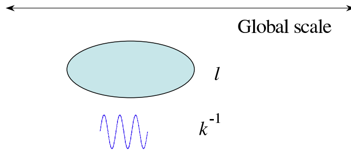
Fig. 9.12. Illustration of the scale length for integral. It is intermediate between the global scale and the microscopic scale of fluctuations.
