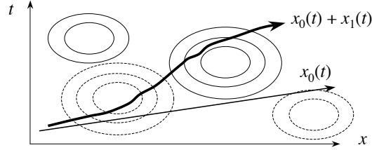
Fig. 3.16. Schematic drawing of the particle orbit in the presence of electric perturbations.
