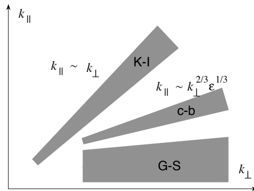
Fig. 9.4. Conceptual illustration for the regimes of Kraichnan-Iroshnikov (K.-I.) spectrum and Goldreich-Sridhar (G-S) spectrum. The critically-balanced regime (c-b) is also illustrated.
