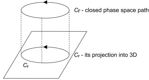
Fig. 8.4. Closed path in a phase space and its projection into the real space.
