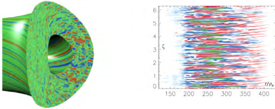
Fig. 6.15. Advance of direct nonlinear simulation in toroidal plasmas. Left: ion-temperature-gradient driven turbulence, and fluctuation on the poloidal cross section of tokamak is illustrated (quoted from (Candy and Waltz)). Right: electron-temperature-gradient driven turbulence, shown on the plane of plasma radius and toroidal angle (quoted from (Lin et al., 2007)).
