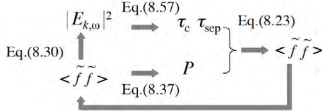
Fig. 8.12. The loop of consistency between the correlation of granulation, radiated electric field, production and separation time.
