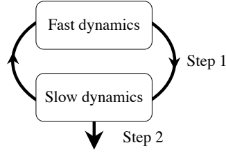
Fig. 6.9. Loop of slow variables and fast variables.
