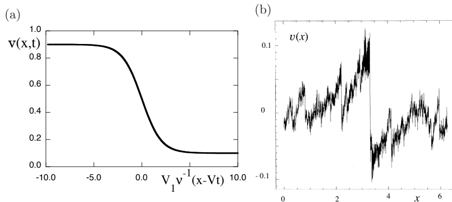
Fig. 6.3. A shock-type solution of the Burgers equation (a). An example of snapshot illustration of v(x, t) for the random-force driven Burgers equation (b) [See details; (Chekholv and Yakhot, 1995)].
