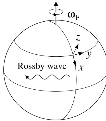
Fig. A1.5. Propagation of Rossby wave in the westward direction.
