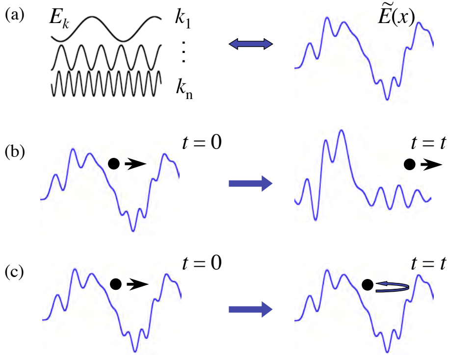
Fig. 3.7. (a) Cartoon of instantaneous pattern of electric field which a particle actually sees. The pattern has an effective duration time of \tau_{ac} . (b) Cartoon showing that for \tau_{ac} < \tau_b , the E -field pattern a particle sees will change before the particle bounces, thus validating the use of unperturbed orbits. (c) Cartoon showing that for \tau_b < \tau_{ac} , the particle will bounce within a field pattern before the pattern changes. In this case, trapping occurs and the use of unperturbed orbits is not valid.
