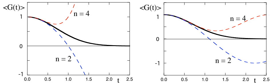
Fig. 6.2. Comparison of \langle G(t) \rangle (solid line) and its truncated approximation (dashed line) for the case of time-series expansion (a). Approximation by use of the moment truncation is shown in (b) by the dashed lines. (For the case of \langle b^2 \rangle = 2 ).
