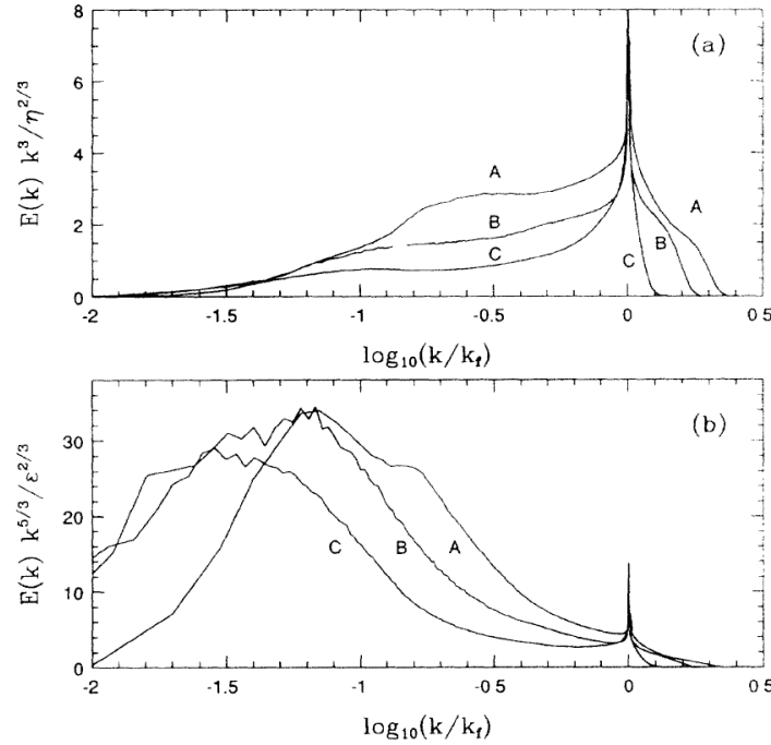
Fig. 2.18. Build-up of a large-scale flow in dual cascade (Borue, 1994). Energy spectra normalized as (a) E(k) k^3 \eta^{-2/3} and (b) E(k) k^{5/3} \varepsilon^{-2/3} as the function of \log_{10}(k/k_f) for three different parameters in simulations. (B and C have finer resolution than A. In C, forcing occurs at finer scale than in B. See (Borue, 1994) for details of parameters.)
