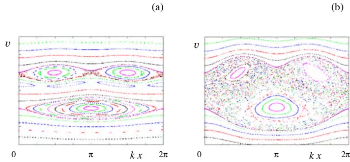
Fig. 3.5. (a) Structure of wave-particle resonance in phase space. The separatrix width is \Delta v \sim (q\phi_i/m)^{1/2} . Particles inside the separatrix (region of libration) undergo periodic motion on iso-energy contours and so are said to be trapped. Particles outside the separatrix circulate. (b) For several waves with distinct phase velocities, multiple resonance islands can co-exist and interact. [Courtesy of Prof. A. Fukuyama].
