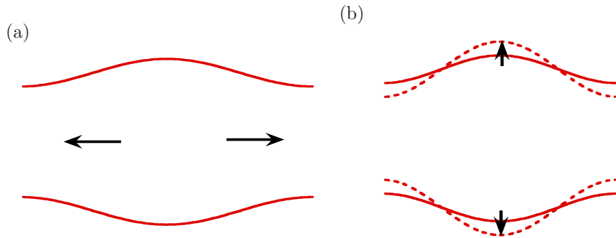
Fig. 9.7. (a) Unperturbed wave train and its envelope. (b) Localized modulational perturbation.
