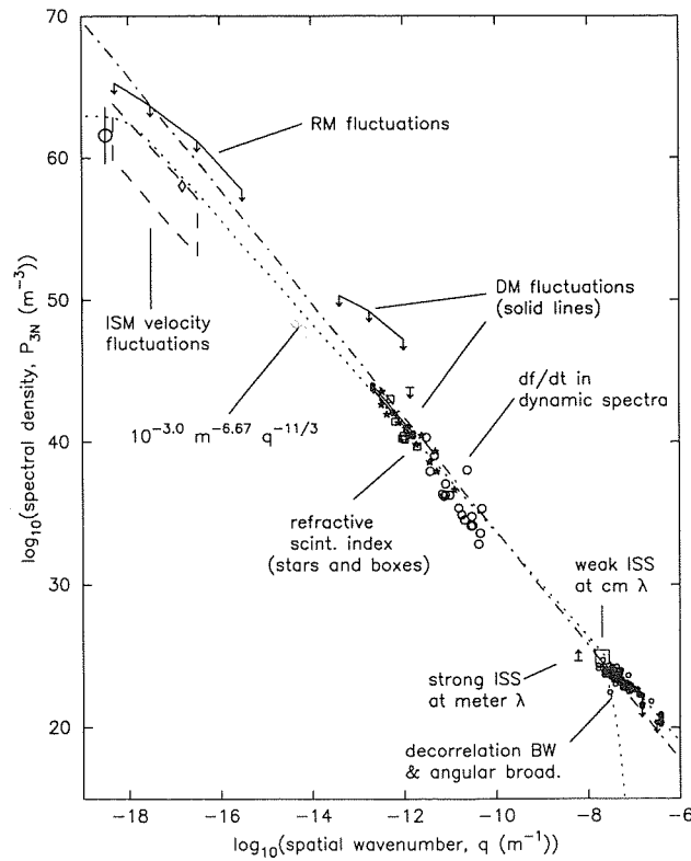
Fig. 9.6. An example of the interstellar density power spectrum in the tenuous phase of the interstellar medium. A power law with index close to the Kolmogorov value of 11/3 is shown by the dotted line [See the original article for details: Quoted from (Armstrong et al., 1995).]
