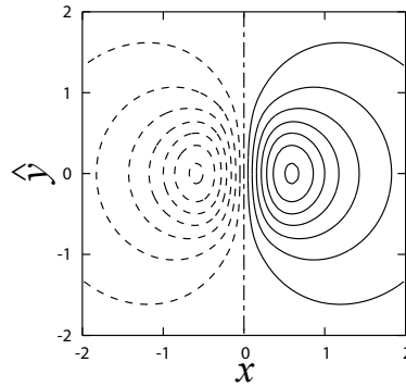
Fig. A1.3. Electrostatic perturbation for the drift wave modon. It propagates in the y -direction. (Parameters: A_m = 1 , v_{**} = (3/2)V_{de} )
