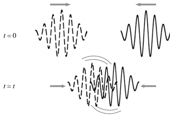
Fig. 9.1. Counter-propagating Alfvén wave streams interact.
