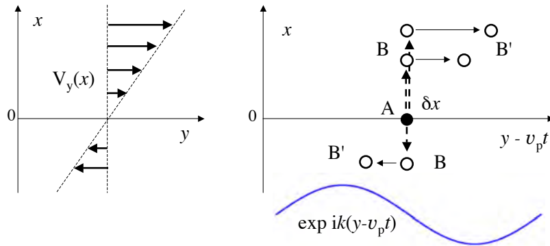
Fig. 4.9. The case of sheared mean flow (a). Accelerated decorrelation occurs via diffusion in the x -direction. The deviation of the plasma elements in the x -direction enhances the rate of phase change, \omega - kV .
