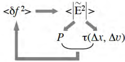
Fig. 8.8. A self-consistent loop between the phasestrophy, radiated electric field fluctuations, production and lifetime of granulations.
