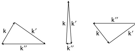
Fig. 5.6. Possible triads where \mathbf{k} + \mathbf{k}' + \mathbf{k}'' = 0
