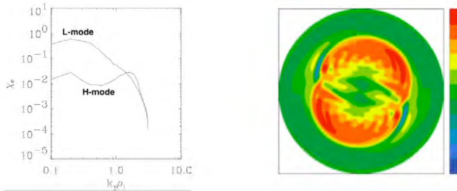
Fig. 6.16. Coexistence of fluctuations at different scale lengths. Left: fine and hyper-fine scale fluctuations coexist, and contribution of each Fourier component to turbulent transport is illustrated (quoted from (Jenko, 2005)). Right: microscopic fluctuation and global instability coexist, and contour of perturbation is shown on the poloidal cross section (quoted from (Yagi et al., 2005)).
