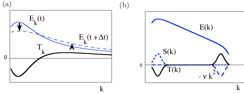
Fig. 6.5. Schematic drawing of the transfer function T_k and the evolution of the spectrum E_k = \langle v_k^2 \rangle (a). Schematic drawing of the stationary state (b).
