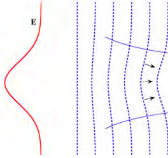
Fig. 7.4. Propagation of a light beam in a nonlinear media with \Delta n > 0 . Phase fronts are shown by dotted lines, and a local direction of propagation is denoted by arrow. Thin lines illustrate knees of the beam intensity profile.
