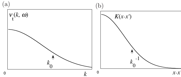
Fig. 6.4. When the response \nu_t(k, \omega) is limited in Fourier space, a nonlocal interaction appears in the coherent drag force.
