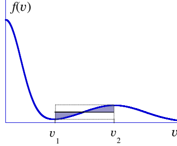
Fig. 3.13. Cartoon of initial and final (plateau) distribution function for resonant region in bump-on-tail instability. Note that quasi-linear diffusion has filled in the initial "hollow" and smoothed out the "bump" centered at v_2 .
