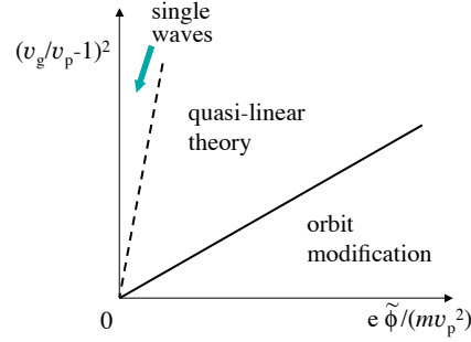
Fig. 3.11. Range of applicability for the quasi-linear theory, Eq.(3.11). Amplitude is normalized by the particle energy at phase velocity on the horizontal axis. Vertical axis shows the magnitude of dispersion, i.e., the difference between the group velocity and phase velocity.
