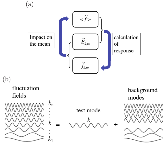
Fig. 4.4. Calculation of the plasma response for given electric field perturbation, and calculation of the evolution of the mean (a). Coupling with test wave and background spectrum is given in (b), depicting the test wave approximation.
