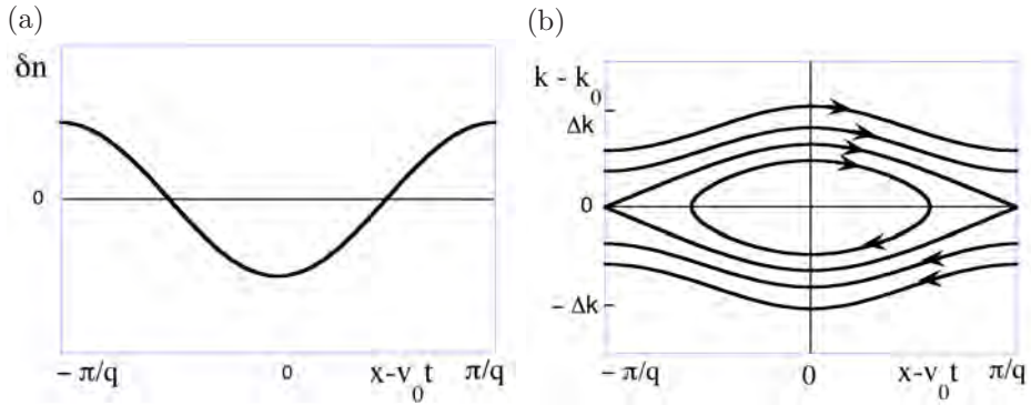
Fig. 7.7. Trapping of quasiparticle in the trough of long-wavelength perturbation. Here v_0 = \Omega/q indicates the phase velocity of long-wavelength mode and k_0 denotes the wavenumber that satisfies the resonance condition v_g = \Omega/q . (a) shows the density perturbation of acoustic mode, and (b) illustrates the trajectory of quasiparticle (plasmon) in the phase space.
