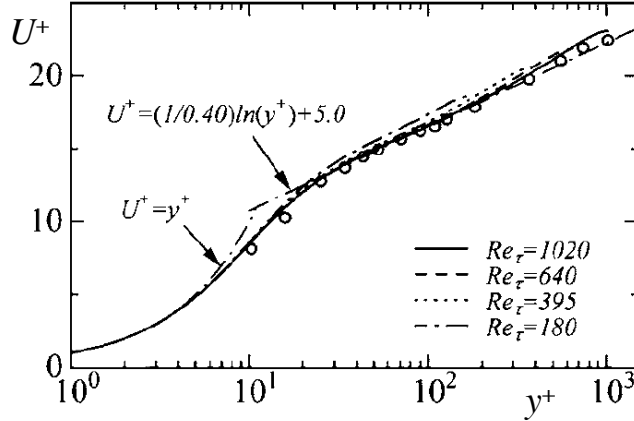
Fig. 2.22. Mean velocity of turbulent channel flows normalized by the friction velocity, U^+ = V(y)/V_* as a function of the normalized distance y^+ = y/y_d . Quoted from (Yoshizawa, 2005), which compiled the lines, DNS (Abe, 2004) and circles, observation (Wei and Willmarth, 1989) at Re_\tau = 1016 . Here, Re_\tau is the Reynolds number defined by use of the friction velocity V_* . Viscous flow near wall, log law and core profile are observed.
