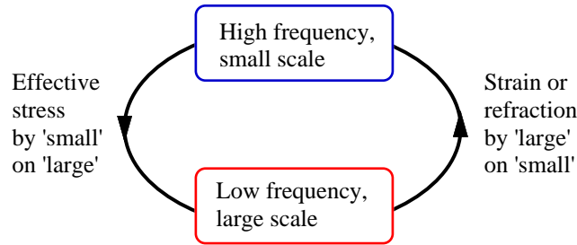
Fig. 7.1. Interaction of small scale-fluctuations and large-scale fluctuations.
