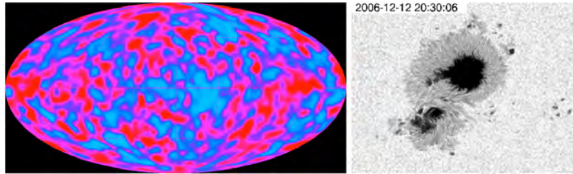
Fig. 1.1. Fluctuations pervade the universe. The cosmic microwave background fluctuations (left). The cosmic microwave background radiation is a remnant of the Big Bang and the fluctuations are the imprint of density contrast in the early universe. [ http://aether.lbl.gov/www/projects/cobe/COBE_Home/DMR_Images.html ] Turbulent dynamics are observed in solar plasmas near the sunspot (right). [Courtesy: Observation by Hinode]
