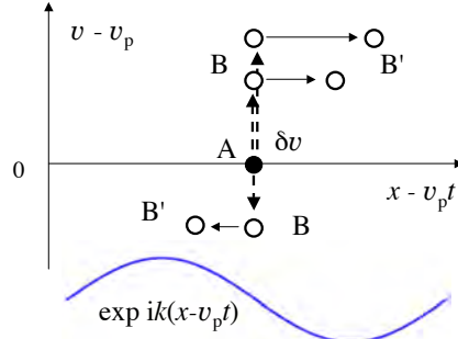
Fig. 4.6. Accelerated decorrelation of resonant particles via diffusion in the velocity space. The deviation of the particle velocity from the phase velocity of the wave enhances the rate of phase change, \omega - kv .
