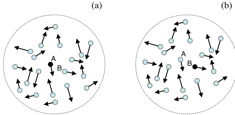
Fig. 2.2. A large number of particles exist within a Debye sphere of particle ‘A’ (shown by black) in (a). Other particles provide a screening on the particle ‘A’. When the particle ‘B’ is chosen as a test particle, others (including ‘A’) produce screening on ‘B’, (b). Each particle acts the role of test particle and the role of screening for other test particle.
