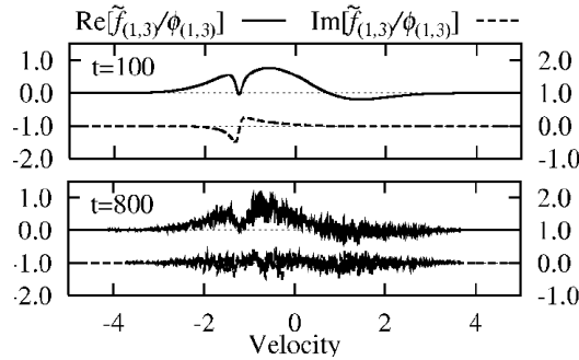
Fig. 8.6. Evolution of the distribution function from the linear phase (top) to the turbulent phase (down) in direct nonlinear simulation. In the turbulent state, small-scale and sharp corrugations are driven until smeared by (small-but-finite) collisions. [Quoted from (Watanabe et al., 2002), which explains details.]
