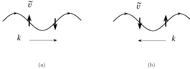
Fig. 9.3. Cross helicity changes sign depending on the propagation direction. In the case that the wave is propagating in the direction of magnetic field (a), the perturbed velocity has opposite sign in comparison to the magnetic field perturbation. The cross helicity is negative. In contrast, when the wave changes the direction of propagation (b), the cross helicity becomes positive.
