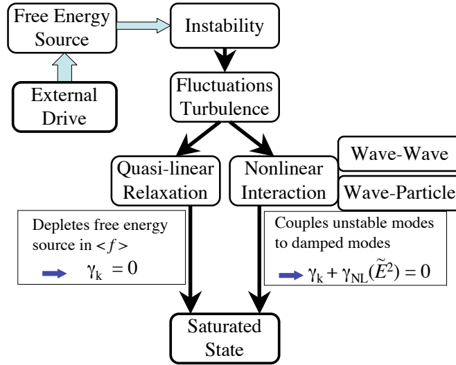
Fig. 4.1. Energy flow in plasma turbulence.
