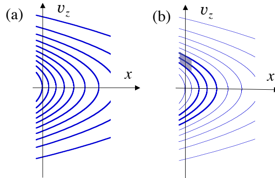
Fig. 3.15. Contour of the mean electron distribution function in the phase space (a). According to the resonance with drift waves, a flattening may occur, and the modification takes place in the level contours of mean distribution, as is illustrated by a shaded region (b).
