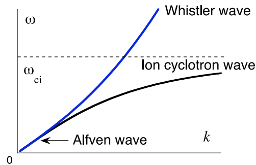
Fig. 9.9. Linear dispersion of a low frequency electromagnetic waves which are propagating in the direction of magnetic field. When the wave length is much longer than the ion-skin depth (or frequency is much smaller than the ion cyclotron frequency), both the right- and left- polarized wave appear as Alfvén waves. In a regime of short wave length, the Alfvén wave continues to whistler wave or ion cyclotron wave.
