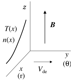
Fig. A1.1. Geometry of inhomogeneous plasma and magnetic field
