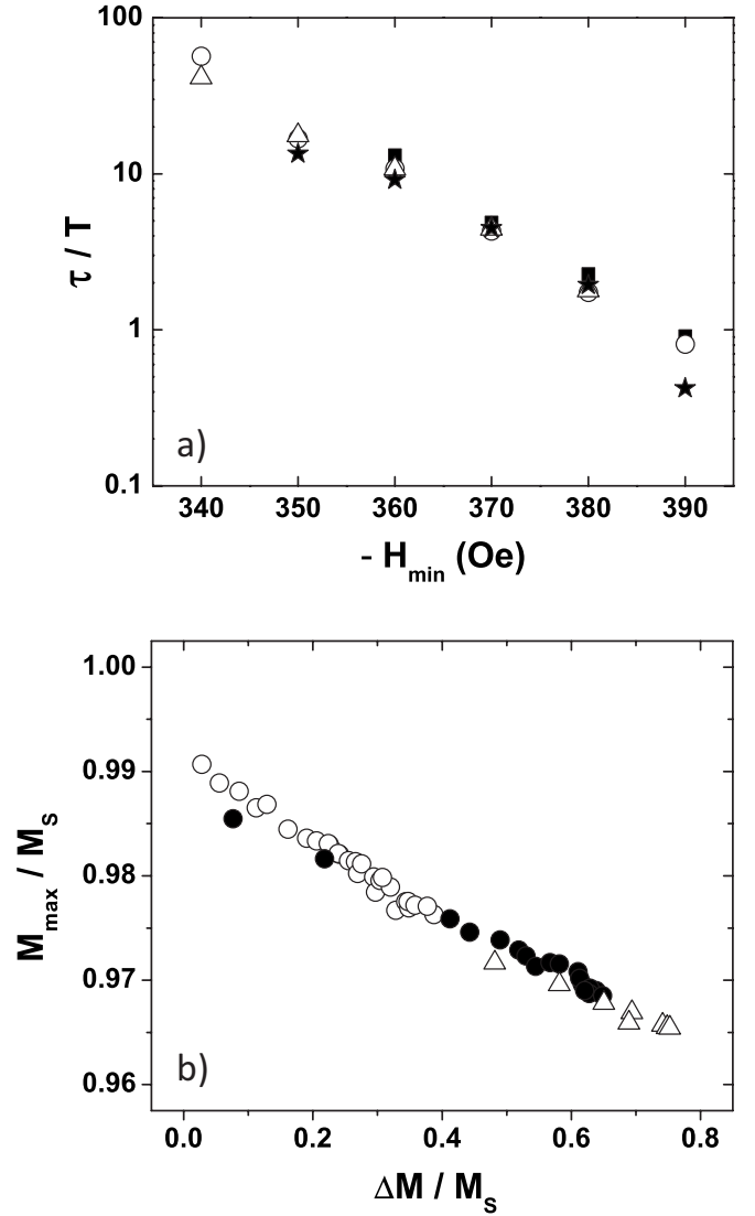
FIG. 6. (a) Relaxation time constant \tau , derived from the least-squares fits of Eq. (5) to experimental data from a (\text{Co/Pd})_8 multilayer, as a function of -H_{\min} for different values of H_{\max} = 500 Oe (■), 450 Oe (○), 400 Oe (△), and H_{\max} = -H_{\min} (★); (b) M_{\max} vs \Delta M data for successive minor loop cycles with -H_{\min} = 360 Oe (○), 370 Oe (●), and 380 Oe (△) and fixed H_{\max} = 500 Oe.
