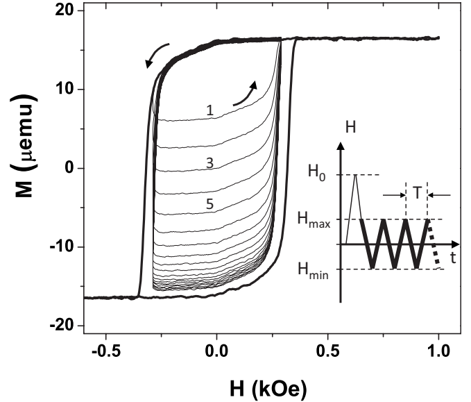
FIG. 1. Field dependence of the magnetization for a (\text{Co}/\text{Pt})_8 multilayer. The thick solid line represents the major loop behavior while the thin solid line shows a sequence of successive minor loops upon applying a symmetric field amplitude of H_{\max} = -H_{\min} = 290 Oe. The first, third, and fifth minor loop are labeled. The inset is a schematic of the H vs t dependence, which was applied for this measurement.
