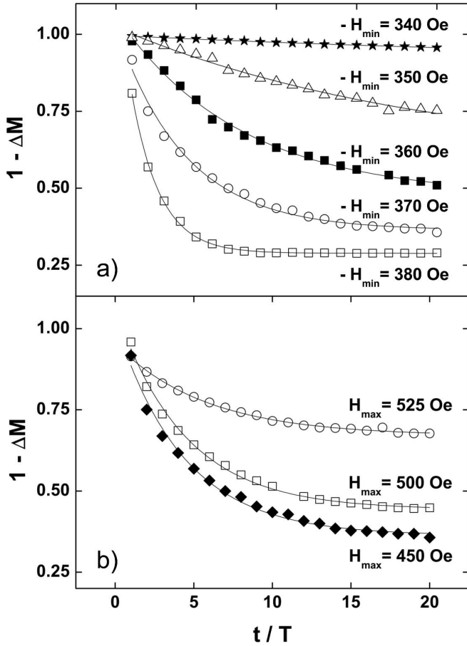
FIG. 5. \Delta M(t) dependence for successive minor loop cycles measured for a (\text{Co/Pd})_8 multilayer upon applying asymmetric field sequences: (a) H_{\max} = 450 Oe for different values of H_{\min} ; (b) -H_{\min} = 370 Oe for different values of H_{\max} .
