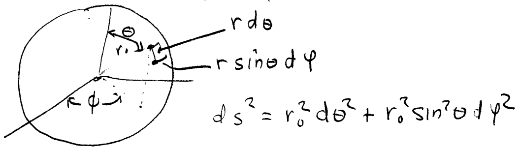
Fig 3: Metric on surface of Earth (2-D)
