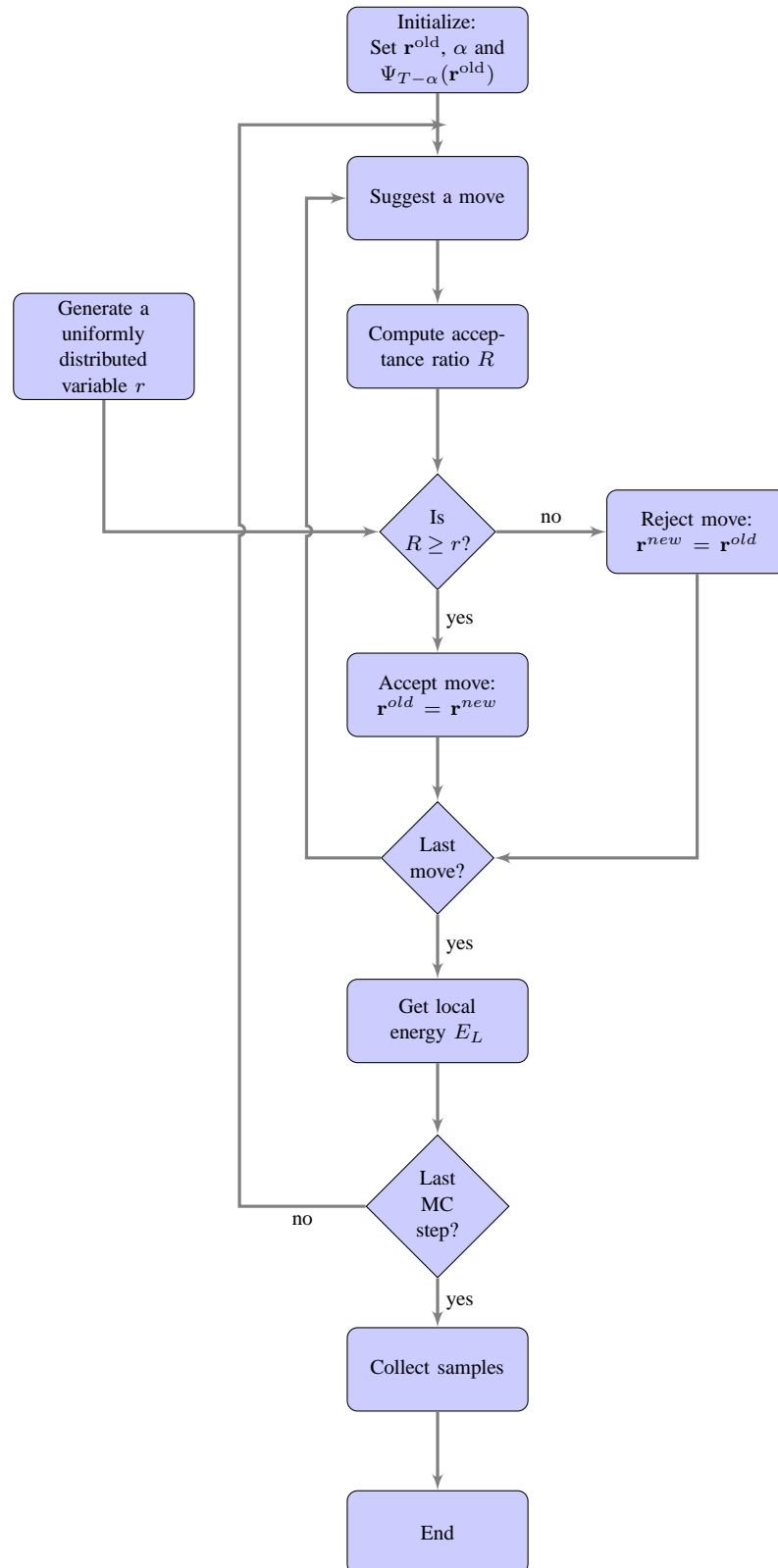
Figure 14.4: Chart flow for the Quantum Variational Monte Carlo algorithm.
