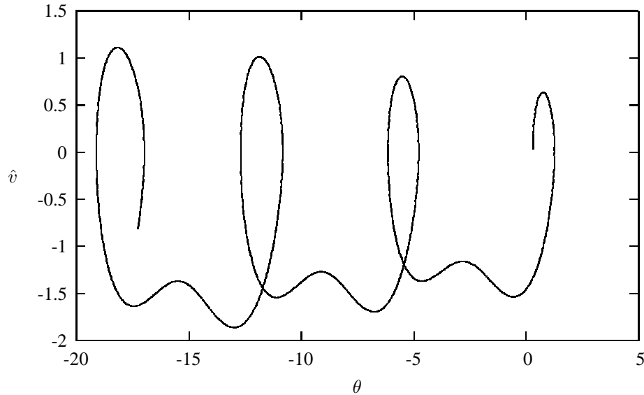
Figure 8.11: Phase-space curve after 10 periods with Q = 2 , \hat{\omega} = 2/3 and \hat{A} = 1.35 . The mass of the pendulum is set equal to 1 kg and its length l = 1 m. The initial velocity is \hat{v}_0 = 0 and \theta_0 = 0.3 .
