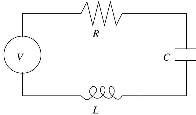
Figure 8.4: Simple RLC circuit with a voltage source V .
