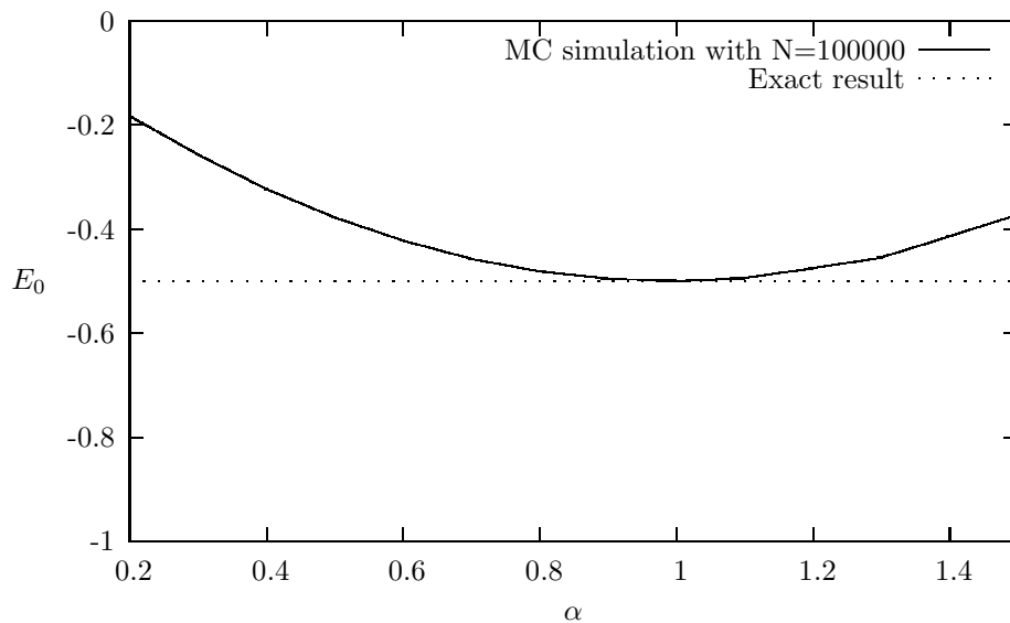
Figure 14.3: Result for ground state energy of the hydrogen atom as function of the variational parameter \alpha . The exact result is for \alpha = 1 with an energy E = -1/2 . See text for further details
