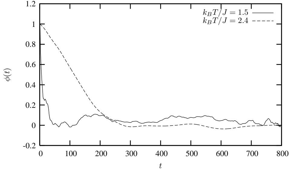
Figure 13.11: Time-autocorrelation function with time t as number of Monte Carlo cycles. It has been normalized with \phi(0) . The calculations have been performed for a 100 \times 100 lattice at k_B T/J = 2.4 with a disordered state as starting point and at k_B T/J = 1.5 with an ordered state as starting point.
