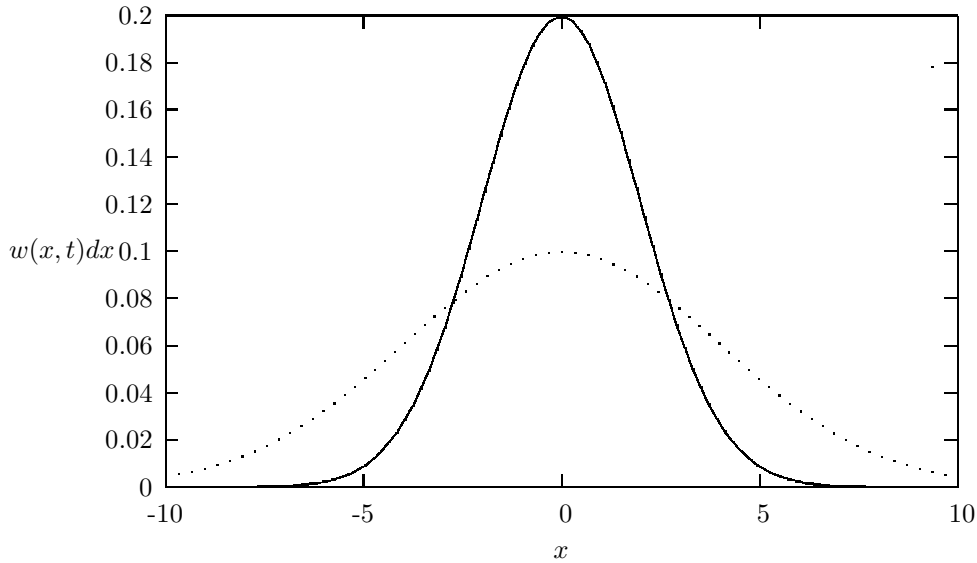
Figure 12.1: Time development of a normal distribution with variance \sigma^2 = 2Dt and with D = 1\text{m}^2/\text{s} . The solid line represents the distribution at t = 2\text{s} while the dotted line stands for t = 8\text{s} .
