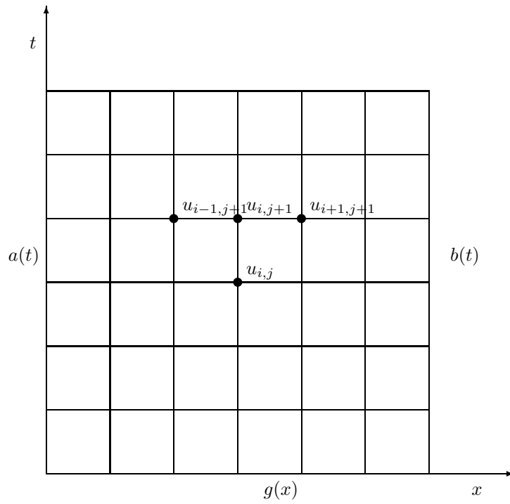
Figure 10.2: Calculational molecule for the implicit scheme.
