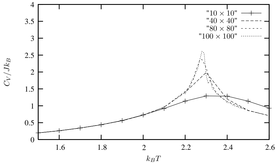
Figure 13.7: Heat capacity per spin as function of the lattice size for the two-dimensional Ising model.
