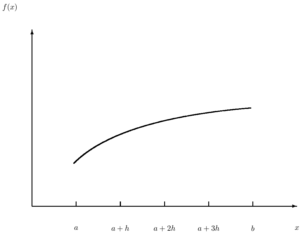
Figure 4.1: The area encribed by the function f(x) starting from x = a to x = b . It is subdivided in several smaller areas whose evaluation is to be approximated by the techniques discussed in the text. The areas under the curve can for example be approximated by rectangular boxes or trapezoids.
