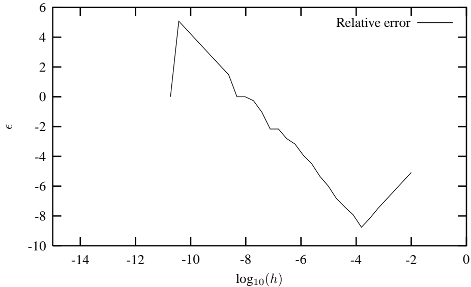
Figure 3.2: Log-log plot of the relative error of the second derivative of \exp(x) as function of decreasing step lengths h . The second derivative was computed for x = 10 in the program discussed above. See text for further details
