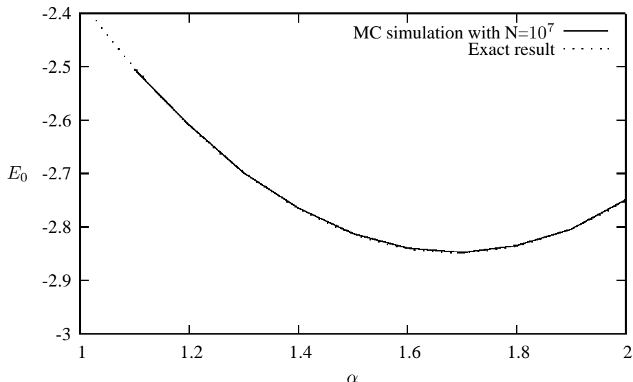
Figure 14.5: Result for ground state energy of the helium atom using Eq. (14.22) for the trial wave function. A total of 10^7 Monte Carlo moves were used with a step length of 1 Bohr radius. Approximately 50% of all proposed moves were accepted. The variance at the minimum is 1.026, reflecting the fact that we do not have the exact wave function. The variance has a minimum at value of \alpha different from the energy minimum. The numerical results are compared with the exact result of Eq. (14.25).
