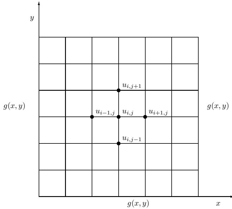
Figure 10.4: Five-point calculational molecule for the Laplace operator of Eq. (10.72). The border \delta\Omega defines the boundary condition u(x, y) = g(x, y) .
