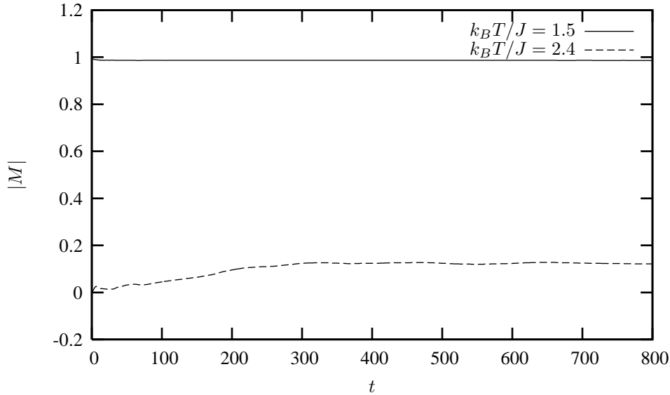
Figure 13.10: Absolute value of the mean magnetisation as function of time t . Time is represented by the number of Monte Carlo cycles. The calculations were performed with a 100 \times 100 lattice for temperatures k_B T / J = 1.5 and k_B T / J = 2.4 . For the lowest temperature, an ordered start configuration was chosen, while for the temperature close to T_C , a disordered configuration was used.
