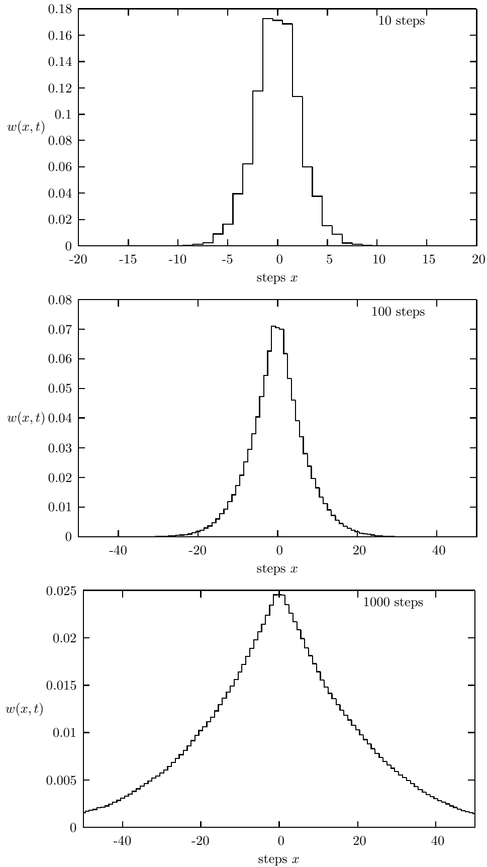
Figure 12.5: Probability distribution for one walker after 10, 100 and 1000 steps.
