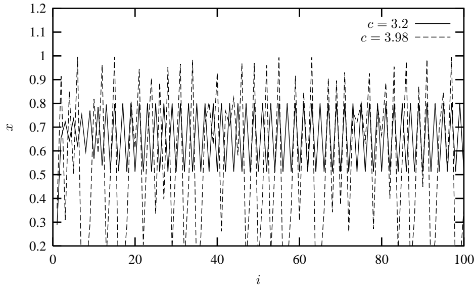
Figure 11.2: Plot of the logistic mapping x_{i+1} = cx_i(1 - x_i) for x_0 = 0.1 and c = 3.2 and c = 3.98 .
