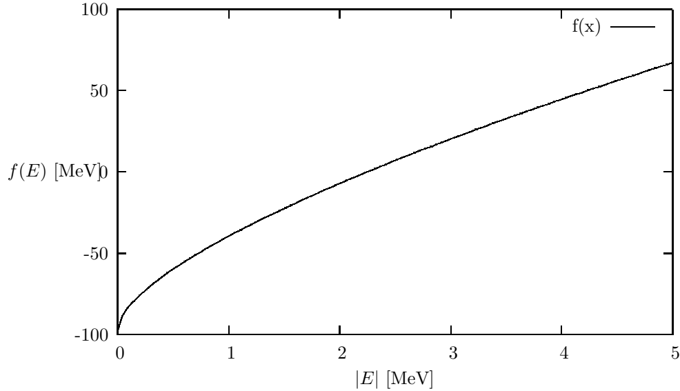
Figure 5.1: Plot of f(E) in Eq. (5.8) as function of energy |E| in MeV. The function f(E) is in units of mega-electronvolts MeV. Note well that the energy E is for bound states.
