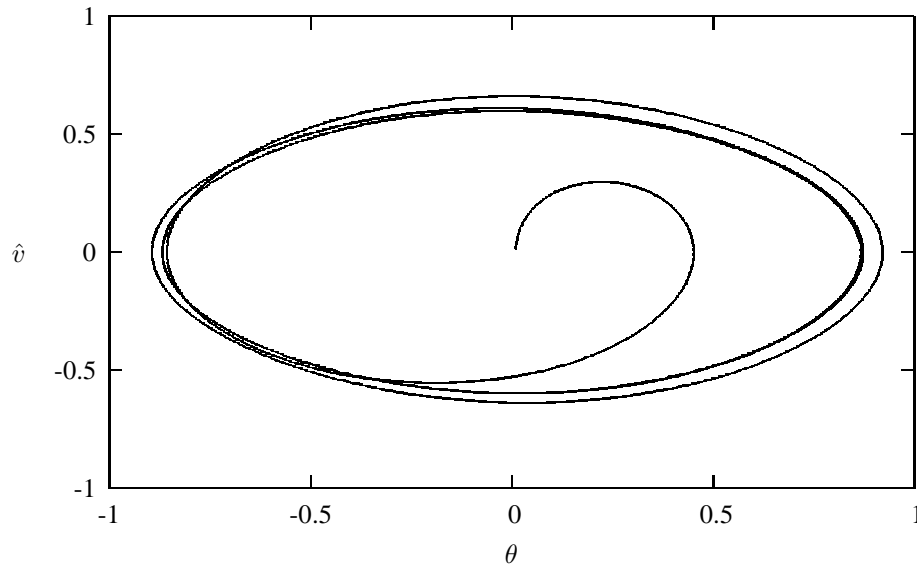
Figure 8.7: Phase-space curve of a linear damped pendulum with Q = 2 , \hat{\omega} = 2/3 and \hat{A} = 0.5 . The initial velocity is \hat{v}_0 = 0 and \theta_0 = 0.01 .
