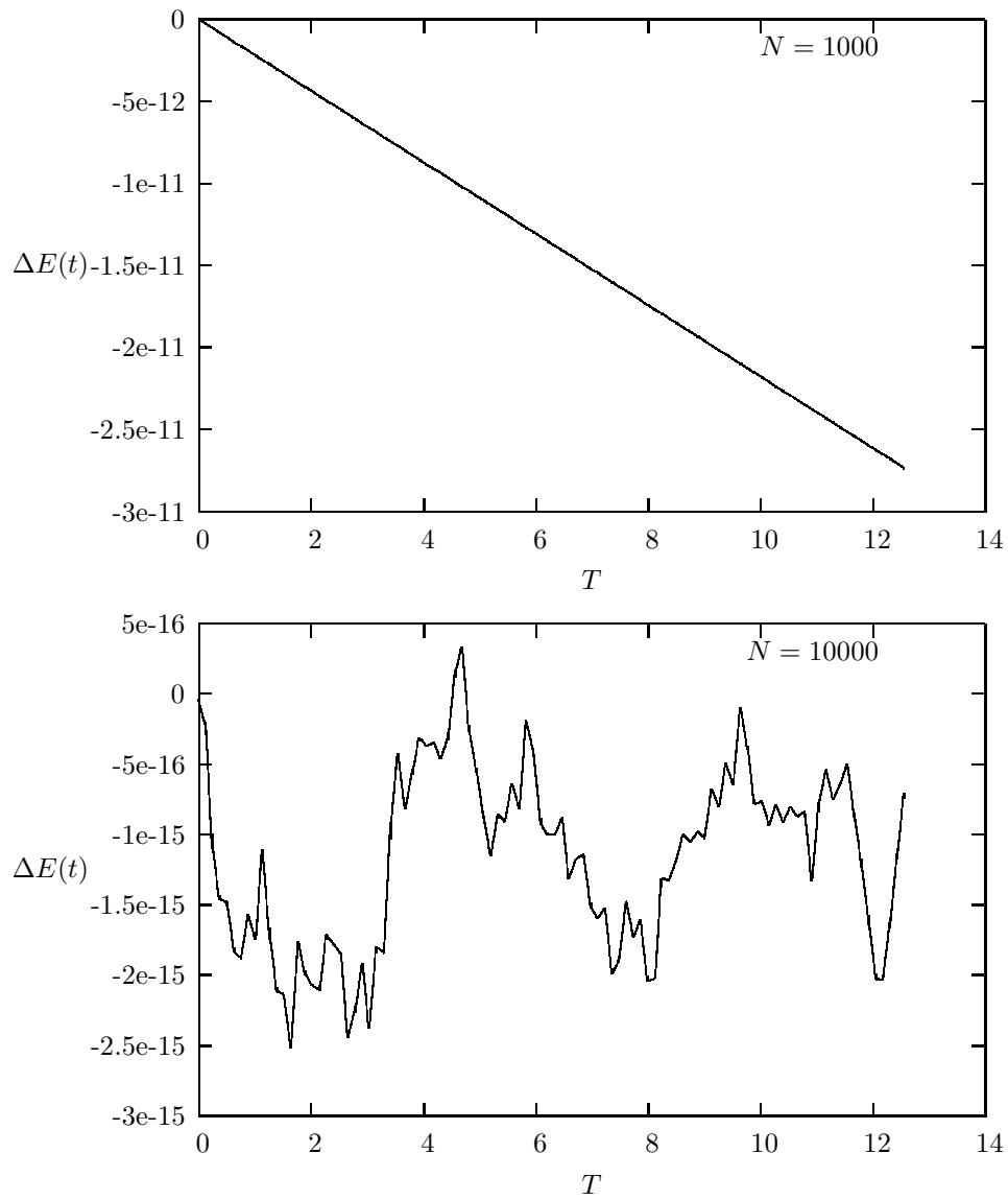
Figure 8.3: Plot of \Delta E(t) = E_0 - E_{\text{computed}} for N = 1000 and N = 10000 time steps up to two periods. The initial position x_0 = 1 m and initial velocity v_0 = 0 m/s. The mass and spring tension are set to k = m = 1 .
