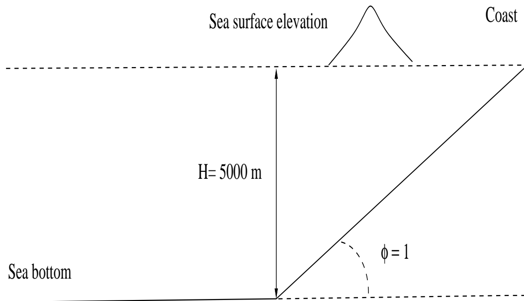
Figure 10.6: The sea bottom towards one of the coastlines has a shape with an inclination of 1 degree. The center of the earthquake is shifted to the right with respect to Fig. 1 as indicated by the exaggerated surface elevation. In this part the surface elevation is moved 40 km to the right.
