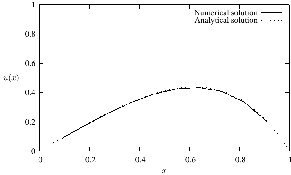
Figure 6.4: Numerical solution obtained with n = 10 compared with the analytical solution.
