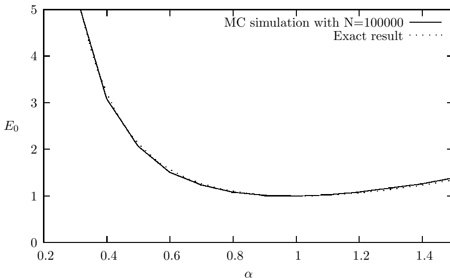
Figure 14.2: Result for ground state energy of the harmonic oscillator as function of the variational parameter \alpha . The exact result is for \alpha = 1 with an energy E = 1 . See text for further details
