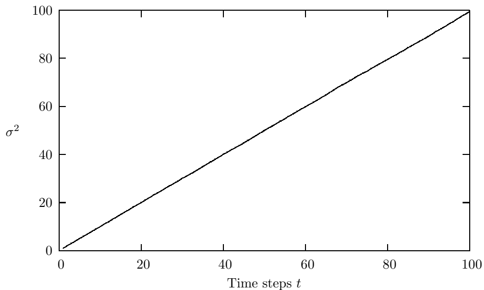
Figure 12.3: Time development of \sigma^2 for a random walker. 100000 Monte Carlo samples were used with the function ran1 and a seed set to -1 .
