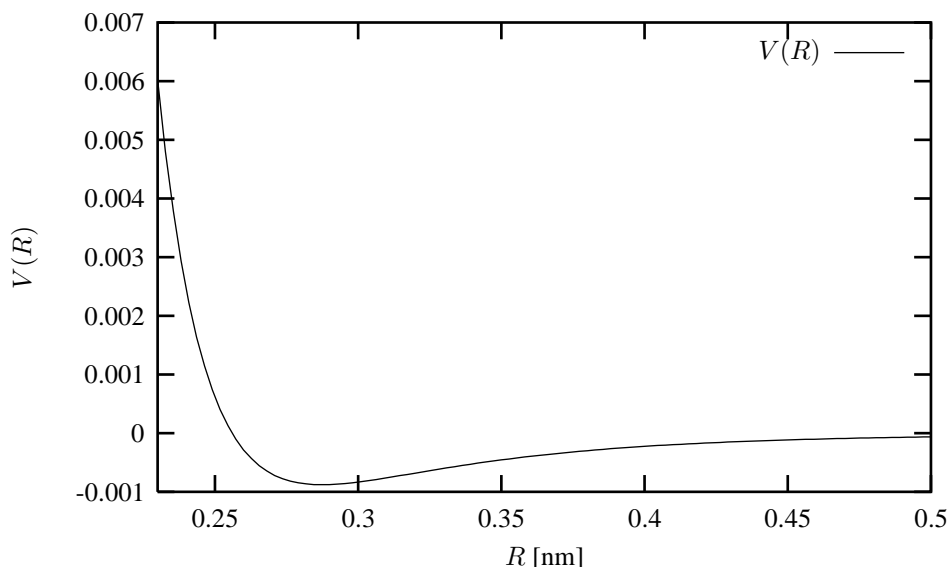
Figure 17.1: Plot for the Van der Waals interaction between helium atoms. The equilibrium position is r_0 = 0.287 nm.
