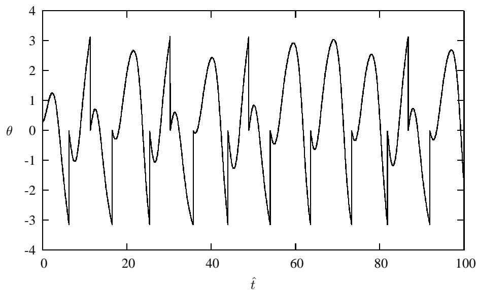
Figure 8.10: Plot of \theta as function of time \tau with Q = 2 , \hat{\omega} = 2/3 and \hat{A} = 1.35 . The mass of the pendulum is set equal to 1 kg and its length to 1 m. The initial velocity is \hat{v}_0 = 0 and \theta_0 = 0.3 . Every time \theta passes the value \pm\pi we reset its value to swing between \theta \in [-\pi, \pi] . This gives the vertical jumps in amplitude.
