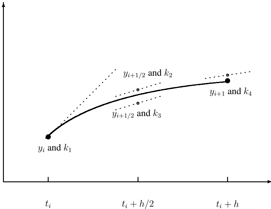
Figure 8.1: Geometrical interpretation of the fourth-order Runge-Kutta method. The derivative is evaluated at four points, once at the initial point, twice at the trial midpoint and once at the trial endpoint. These four derivatives constitute one Runge-Kutta step resulting in the final value for y_{i+1} = y_i + 1/6(k_1 + 2k_2 + 2k_3 + k_4) .
