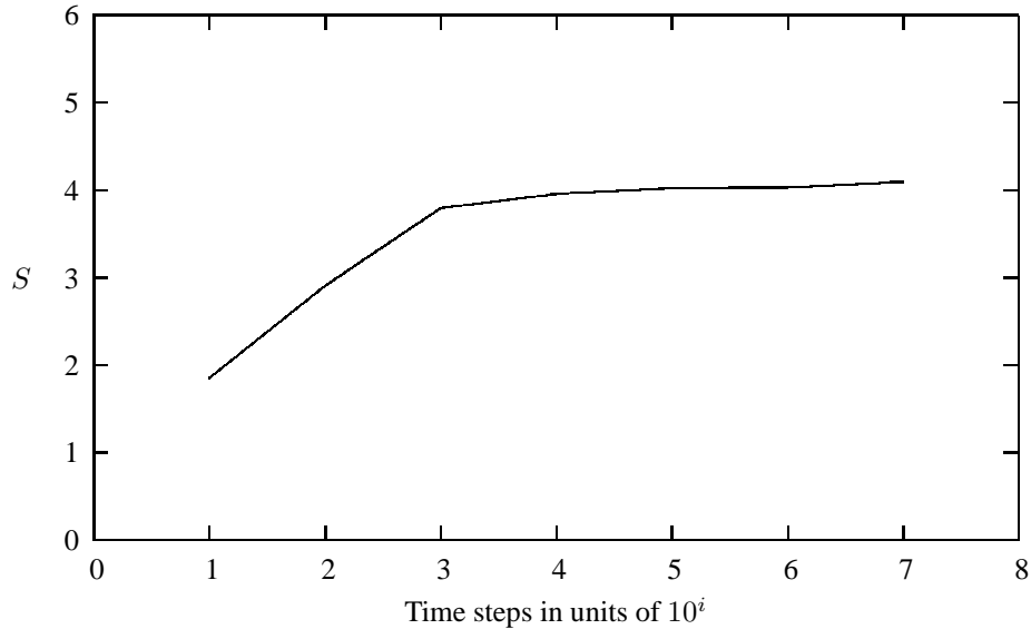
Figure 12.6: Entropy S_j as function of number of time steps j for a random walk in one dimension. Here we have used 100 walkers on a lattice of length from L = -50 to L = 50 employing periodic boundary conditions meaning that if a walker reaches the point x = L + 1 it is shifted to x = -L and if x = -L it is shifted to x = L .
