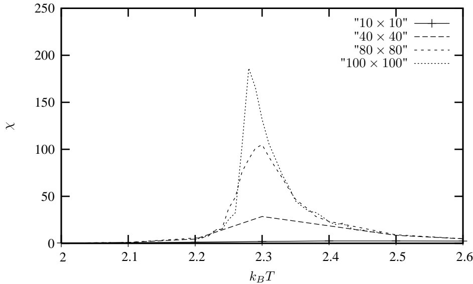
Figure 13.8: Susceptibility per spin as function of the lattice size for the two-dimensional Ising model. Note that we have computed the susceptibility as \xi = (\langle M^2 \rangle - \langle |M| \rangle^2) / k_b T .
