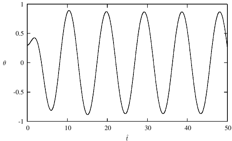
Figure 8.8: Plot of \theta as function of time \tau with Q = 2 , \hat{\omega} = 2/3 and \hat{A} = 0.5 . The mass of the pendulum is set equal to 1 kg and its length to 1 m. The initial velocity is \hat{v}_0 = 0 and \theta_0 = 0.3 .
