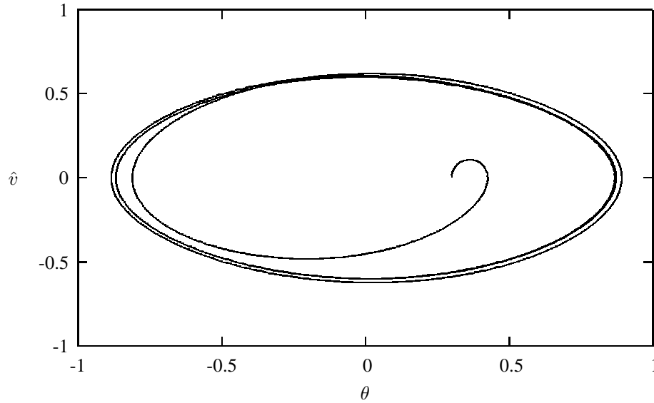
Figure 8.9: Phase-space curve with Q = 2 , \hat{\omega} = 2/3 and \hat{A} = 0.5 . The mass of the pendulum is set equal to 1 kg and its length l = 1 m.. The initial velocity is \hat{v}_0 = 0 and \theta_0 = 0.3 .
