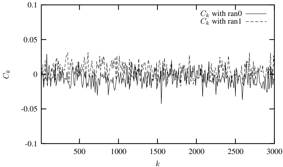
Figure 11.3: Plot of the auto-correlation function C_k for various k -values for N = 10000 using the random number generators ran0 and ran1 .
