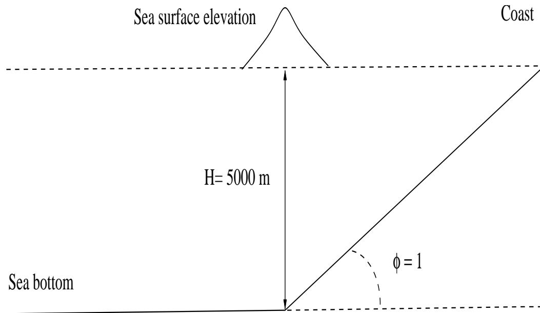
Figure 10.5: The sea bottom towards one of the coastlines has a shape with an inclination of 1 degree and depth where the earthquake takes place of 5000 m. The surface elevation is exaggerated on the figure.
