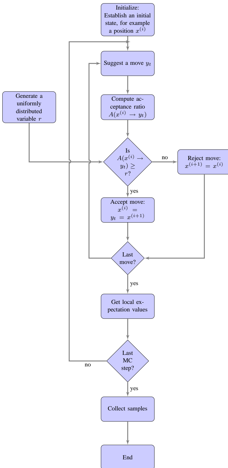
Figure 12.7: Chart flow for the Quantum Variational Monte Carlo algorithm.
