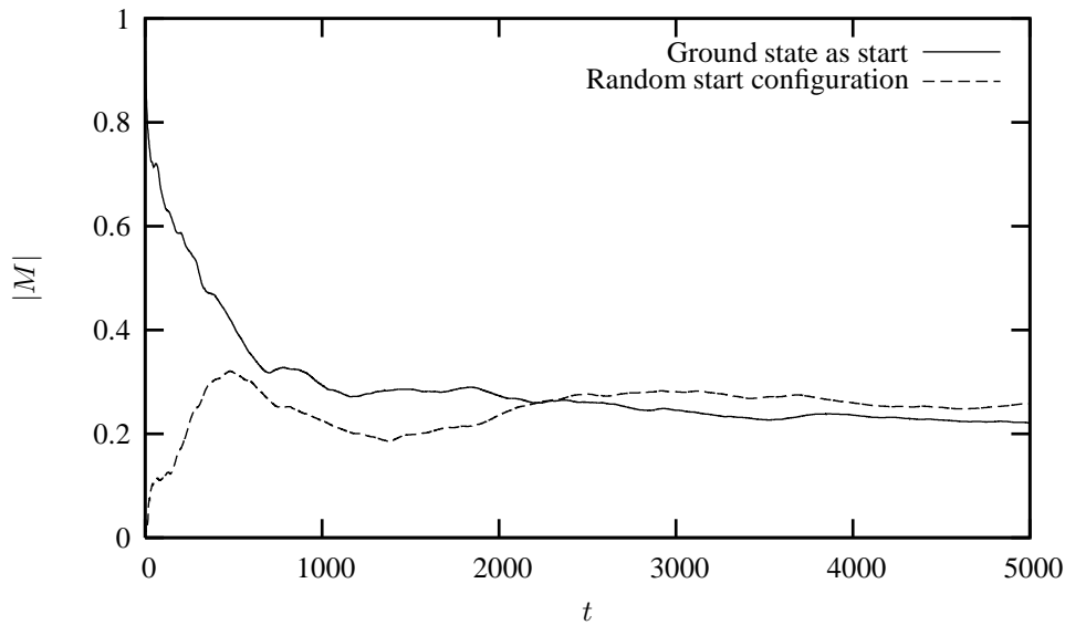
Figure 13.9: Absolute value of the mean magnetisation as function of time t . Time is represented by the number of Monte Carlo cycles. The calculations have been performed with a 40 \times 40 lattice for a temperature k_B T/J = 2.4 . Two start configurations were used, one with a random orientation of the spins and one with an ordered orientation, which corresponds to the ground state of the system.
