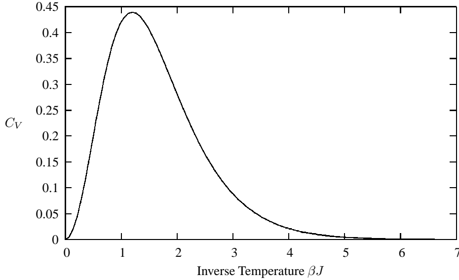
Figure 13.3: Heat capacity per spin ( C_V/(N-1)k_B ) as function of inverse temperature \beta for the one-dimensional Ising model.
