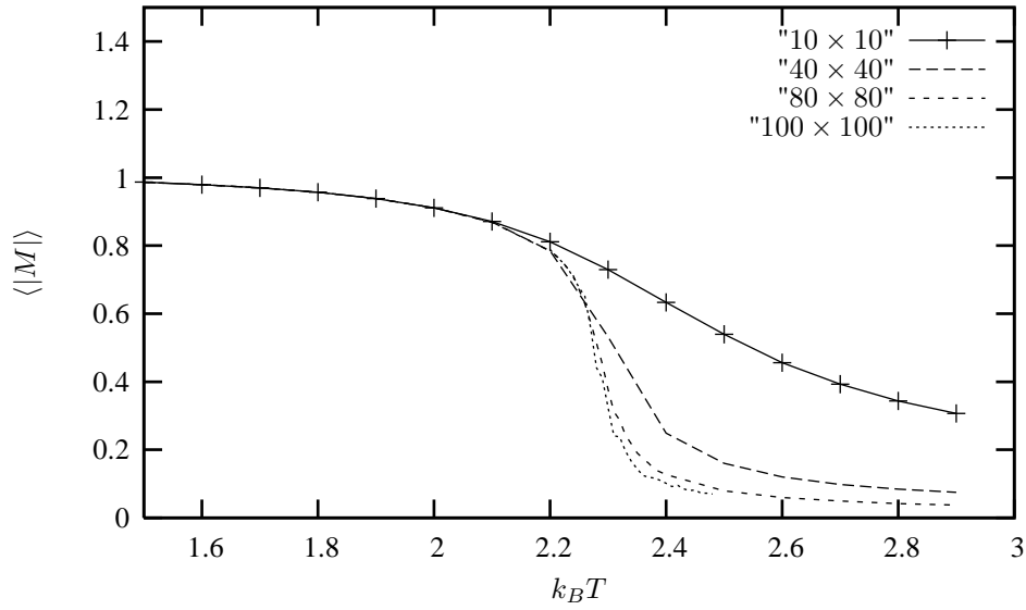
Figure 13.6: Absolute value of the average magnetization per spin as function of the lattice size for the two-dimensional Ising model.
