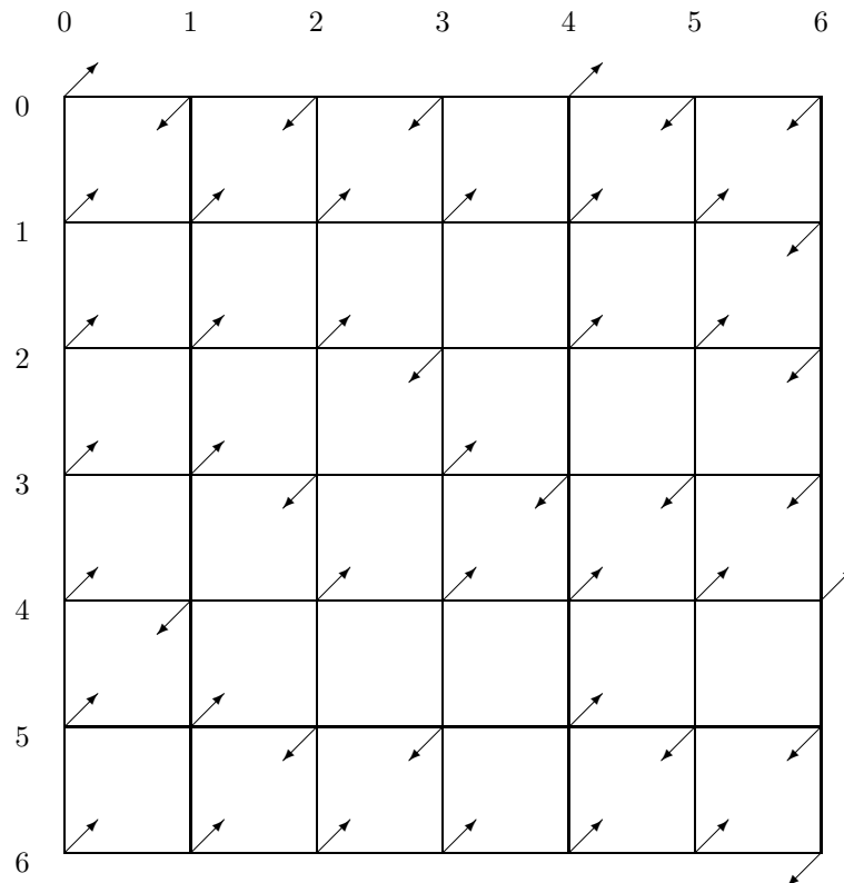
Figure 13.4: Example of a two-dimensional 7 \times 7 lattice with spins pointing either up or down. The variable spin_matrix[1][0] takes the value +1 while spin_matrix[0][6] is -1 .
