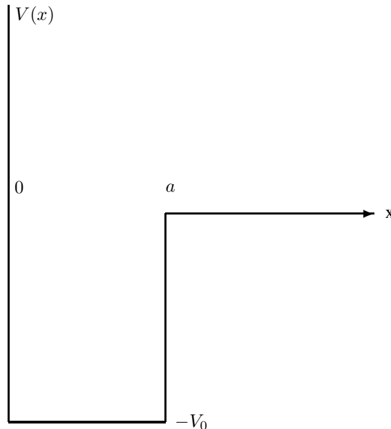
Figure 9.1: Example of a finite box potential with value -V_0 in 0 < x \leq a , infinitely large for x \leq 0 and zero else.
