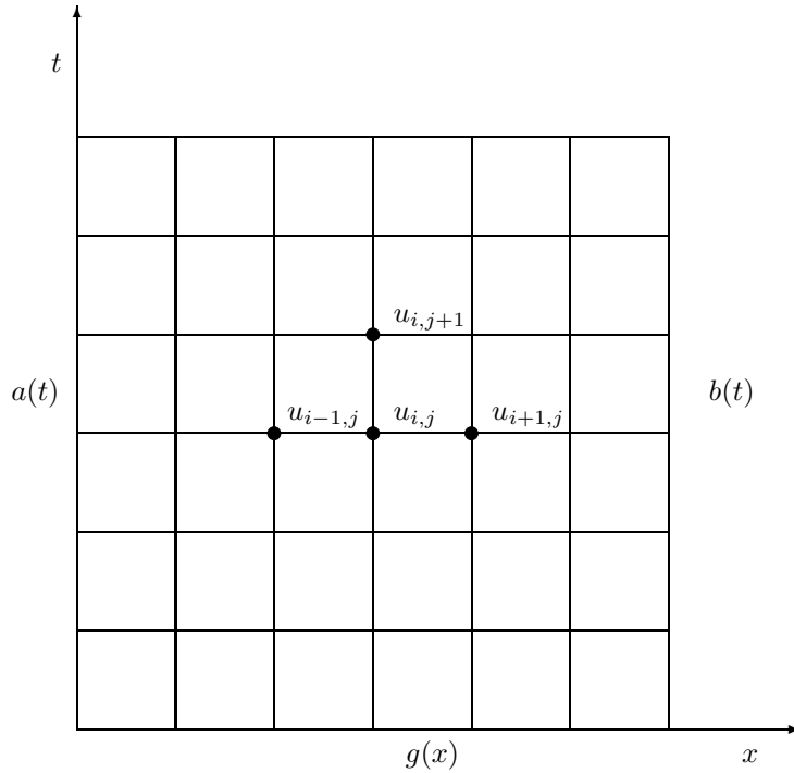
Figure 10.1: Discretization of the integration area used in the solution of the 1 + 1-dimensional diffusion equation. This discretization is often called calculational molecule.
