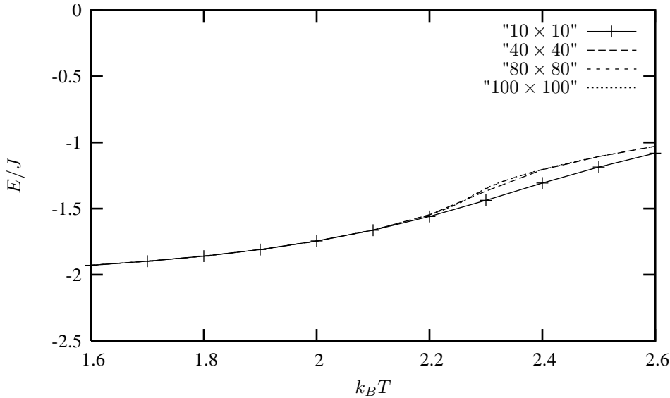
Figure 13.5: Average energy per spin as function of the lattice size for the two-dimensional Ising model.
