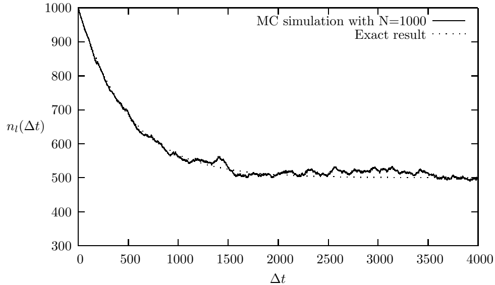
Figure 11.1: Number of particles in the left half of the container as function of the number of time steps. The solution is compared with the analytic expression. N = 1000 .
