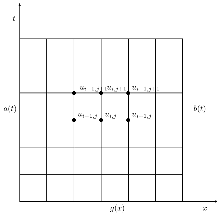
Figure 10.3: Calculational molecule for the Crank-Nicolson scheme.
