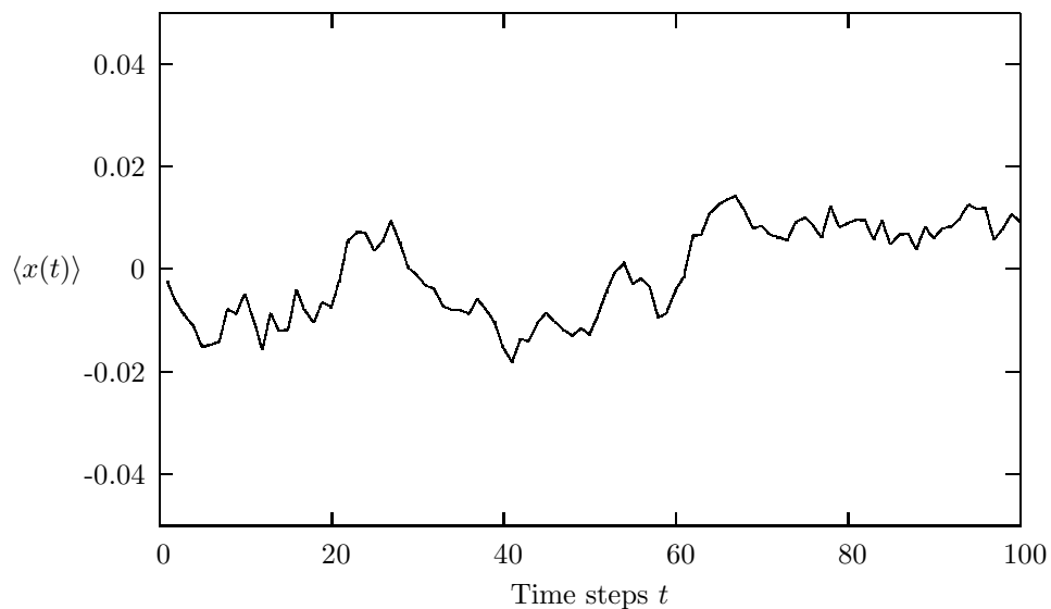
Figure 12.4: Time development of \langle x(t) \rangle for a random walker. 100000 Monte Carlo samples were used with the function ran1 and a seed set to -1 .
