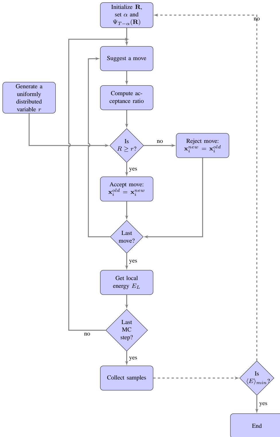
Figure 16.1: Optimization of the trial wave function \Psi_{trial}(\alpha) and minimization of the energy with respect to the variational parameters.
