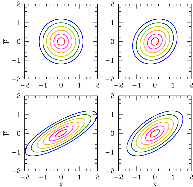
Figure 8.1: Level sets for a sample f(\bar{x}, \bar{p}, \bar{t}) = A e^{-\frac{1}{2}(\bar{x}-\bar{p}\bar{t})^2} e^{-\frac{1}{2}\bar{p}^2} , for values f = A e^{-\frac{1}{2}\alpha^2} with \alpha in equally spaced intervals from \alpha = 0.2 (red) to \alpha = 1.2 (blue). The time variable \bar{t} is taken to be \bar{t} = 0.0 (upper left), 0.2 (upper right), 0.8 (lower right), and 1.3 (lower left).
