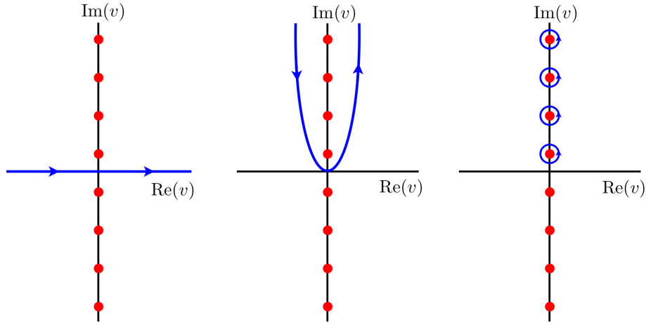
Figure 5.14: Deformation of the complex integration contour in eqn. 5.219.
