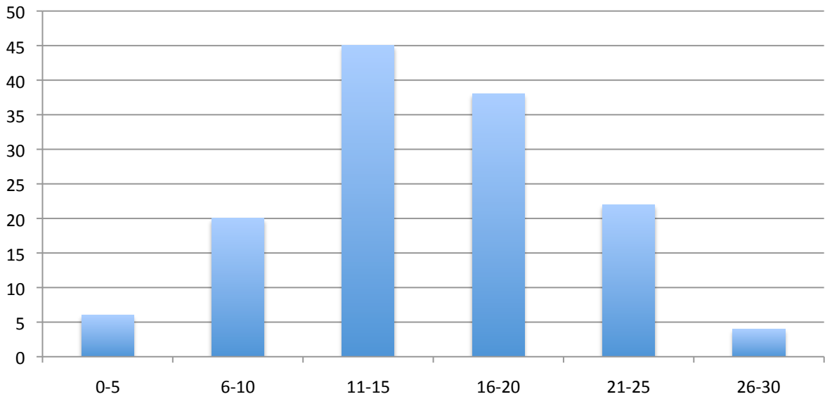
Quiz 5 Histogram
