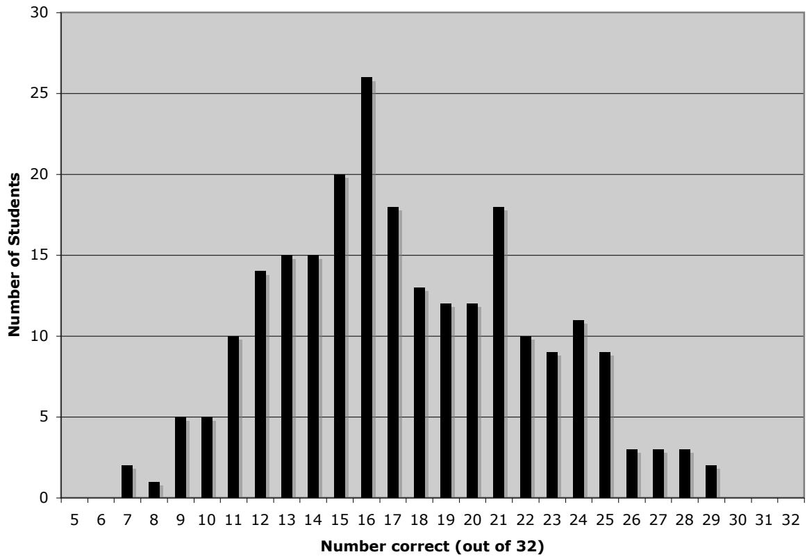
Physics 2A(a) Final Exam Distribution
