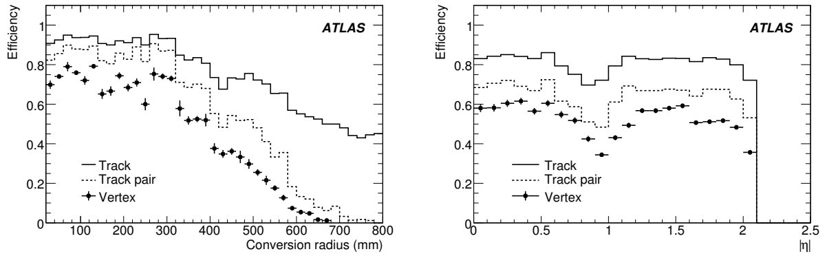
Figure 14: Conversion reconstruction efficiency for conversions from 20 GeV p_T photons as a function of conversion radius (left) and pseudorapidity (right). The solid histograms show the track reconstruction efficiency, the dashed histograms show the track-pair reconstruction efficiency, and the points with error bars show the conversion vertex reconstruction efficiency.
