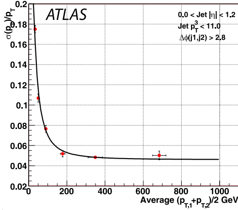
Figure 27: The effective jet energy resolution for cone 0.7 jets after removing soft radiation effects by subtracting in quadrature \sigma_\eta from \sigma_\psi .
