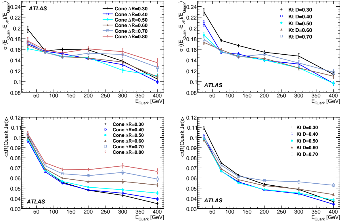
Figure 1: Studies of b -jet resolution: width of (E_{quark} - E_{jet})/E_{quark} and average of \Delta R(\text{Quark}, \text{Jet}) for Cone and k_T with different jet sizes.
