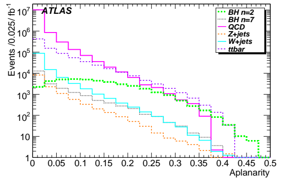
Figure 7: Different event shape variables for black hole samples and backgrounds. They are normalised to the integrated luminosity of 1 \text{ fb}^{-1} .
