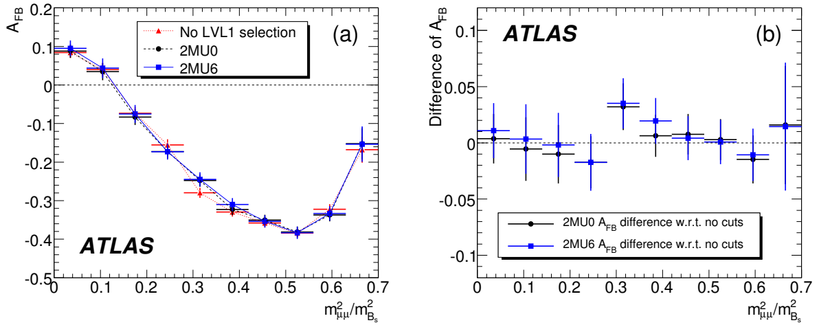
Figure 7: (a) Forward-Backward asymmetry in B_s^0 \rightarrow \mu^+ \mu^- \phi events: no level-1 selection (filled triangles), triggered by 2MU0 (filled circles) and by 2MU6 (open squares). (b) deviation between A_{FB} 's with and without triggers ( A_{FB}[2MUx] - A_{FB}[no\ selection] ): 2MU0 (filled circles) and 2MU6 (open squares).
