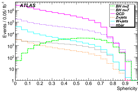
Figure 7: Different event shape variables for black hole samples and backgrounds. They are normalised to the integrated luminosity of 1 \text{ fb}^{-1} .
