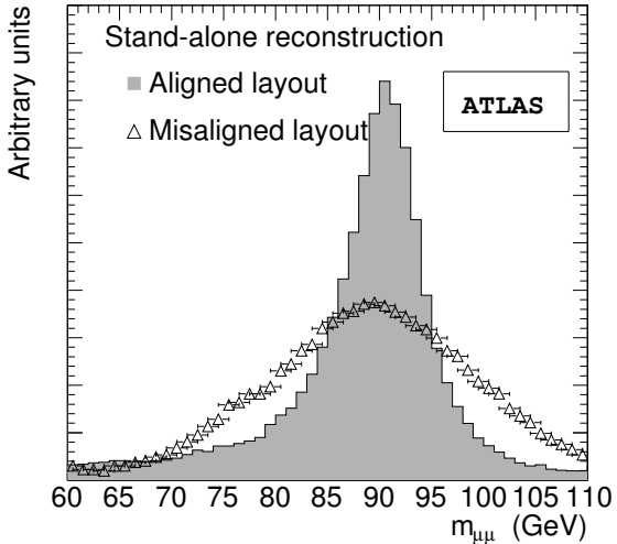
Figure 8: Reconstructed Z boson mass distributions for an aligned and a misaligned ( \sigma_m^{scale} = 1 ) muon spectrometer layout.
