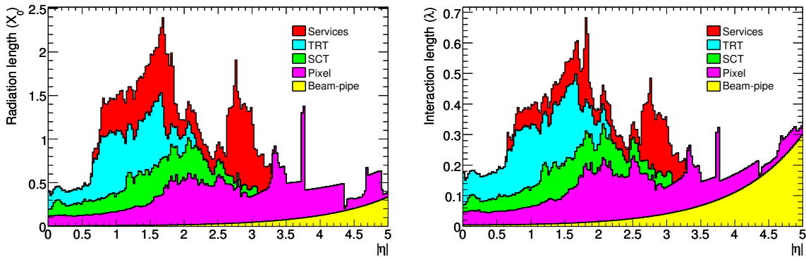
Figure 3: Material distribution ( X_0, \lambda ) at the exit of the ID envelope, including the services and thermal enclosures. The distribution is shown as a function of |\eta| and averaged over \phi . The breakdown indicates the contributions of external services and of individual sub-detectors, including services in their active volume.
