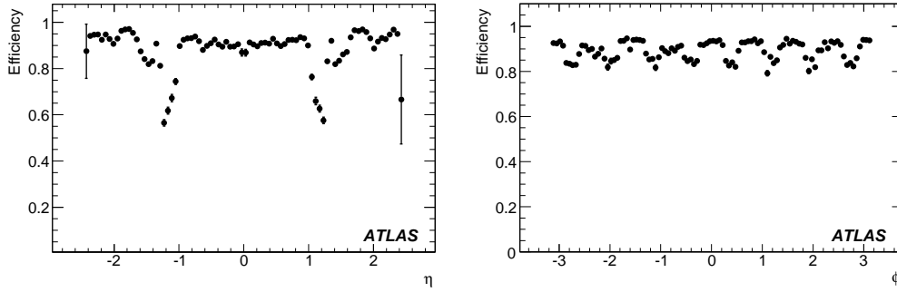
Figure 15: Efficiency of MuId Combined as a function of \eta (left) and of \phi (right) for 6 GeV muons.
