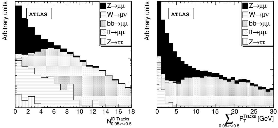
Figure 8: Distributions of the muon isolation variables for signal and backgrounds after all selection cuts. Left : track multiplicity within \Delta R = 0.5 around the muon. Right : total transverse momentum of these tracks.
