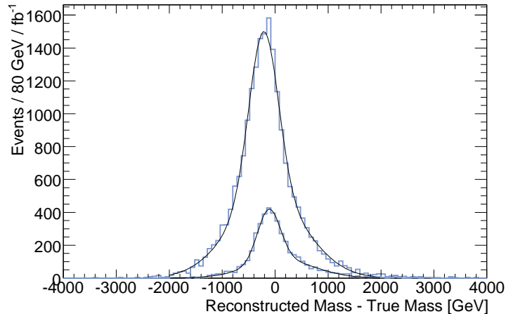
Figure 22: Black hole mass resolution distributions and their fits to double Gaussian functions, using a \Sigma |p_T| and lepton requirement ( 1 \text{ fb}^{-1} ). The upper curve is without a \cancel{E}_T cut. The lower curve has an additional requirement on \cancel{E}_T < 100 \text{ GeV} .
