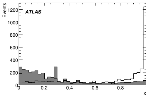
Figure 4: Distribution of the discriminant variable X based on the combination of the transverse and longitudinal impact parameter significances for b -jets and u -jets (dark area) at L2.
