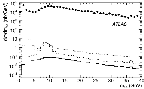
Figure 4: Expected differential cross section for low-mass electron pairs using the 2EM3 trigger menu item after L1 selection for J/\psi decays (dotted histogram), \Upsilon decays (dashed histogram), Drell-Yan production (solid histogram) and expected background (full circles). The invariant mass is reconstructed with calorimeter only information available at L1.
