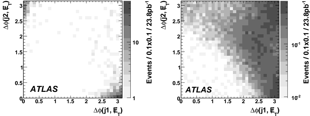
Figure 2: The |\Delta\phi(j_1, E_T^{\text{miss}})| - |\Delta\phi(j_2, E_T^{\text{miss}})| plane for QCD multijet (left) and SUSY SU3 events (right) passing SUSY jet cuts and E_T^{\text{miss}} > 100 GeV.
