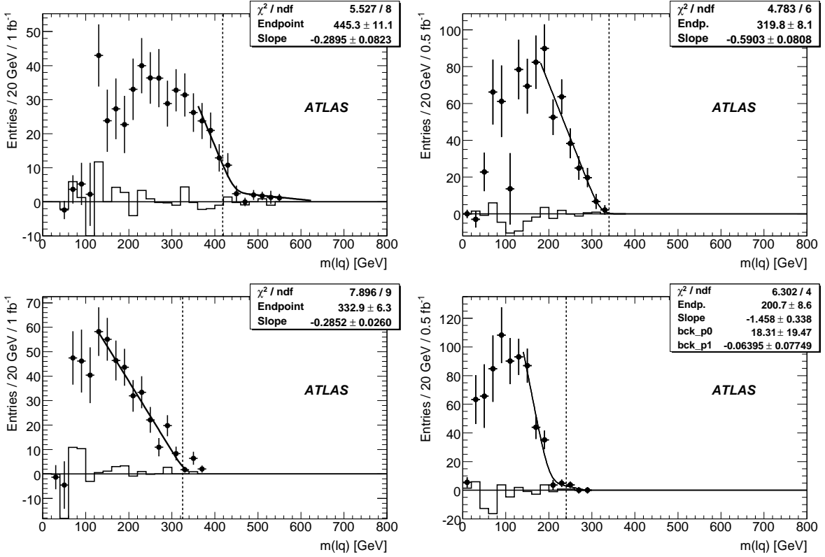
Figure 5: Efficiency-corrected flavour-subtracted distributions of m_{lq}^{(\text{high})} (top) and m_{lq}^{(\text{low})} (bottom) for SU3 (left) with 1 \text{ fb}^{-1} and SU4 (right) with 0.5 \text{ fb}^{-1} of integrated luminosity. The points with error bars show SUSY plus Standard Model, the solid histogram shows the Standard Model contribution alone. The fitted function is superimposed, the vertical line indicates the theoretical endpoint value.
