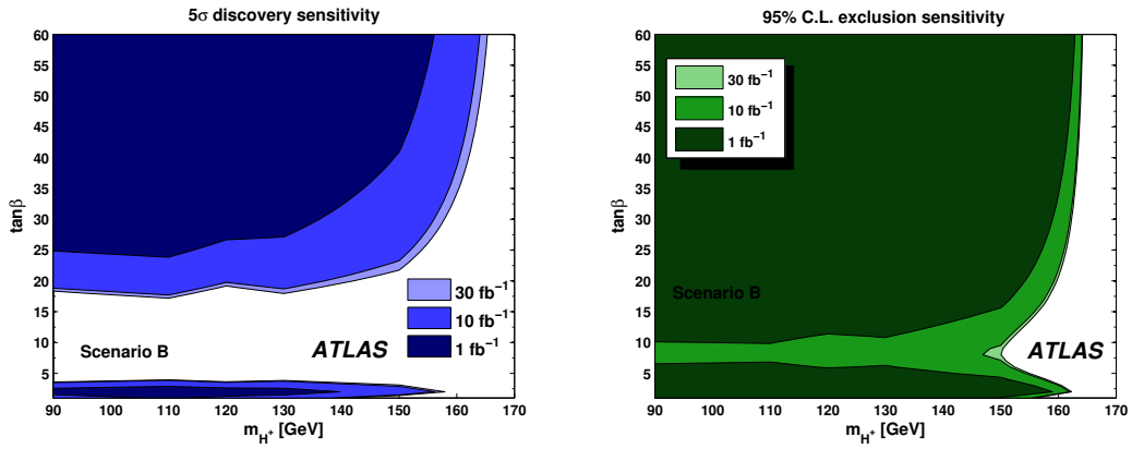
Figure 2: t\bar{t} \rightarrow bH^+bW \rightarrow b\tau(had)\nu bq\bar{q} : Discovery (left) and exclusion contour (right) for Scenario B ( m_h -max) [1]. Systematic and statistical uncertainties are included. The systematic uncertainty is assumed to be 10% for the background, and 24% for the signal (see Sections 5.2 and 5.1). The lines indicate a 5\sigma significance for the discovery and a 95% CL for the exclusion contour.
