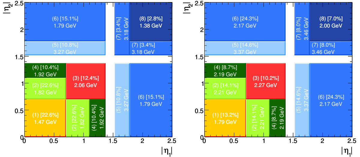
Figure 12: Regions of photon pseudorapidities with different invariant mass resolutions for unconverted photons (left) and at least one converted photon (right). The text per box denotes the region number, the percentage of events occurring in the region and the RMS of the diphoton invariant mass for H \rightarrow \gamma\gamma events. To simplify the likelihood model, events with photons in regions (1) and (8) are merged and represent category “good” (signal fraction 24%), events in regions (2), (3), (4) and (6) correspond to category “medium” (60%), and regions (5) and (7) are “bad” (15%).
