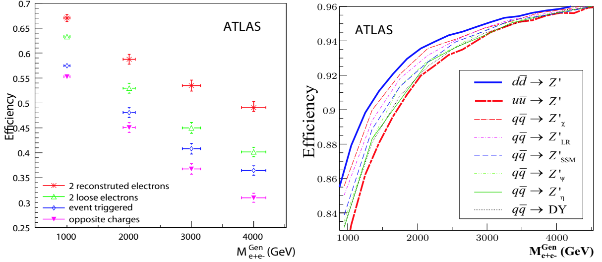
Figure 7: Z'_{\chi} \rightarrow e^+e^- selection efficiency as a function of the generated invariant mass. Left: all selections, normalized to events in the geometrical acceptance; right: |\eta| < 2.5 criteria for u\bar{u} and d\bar{d} events separately and for different Z' models (generator level).
