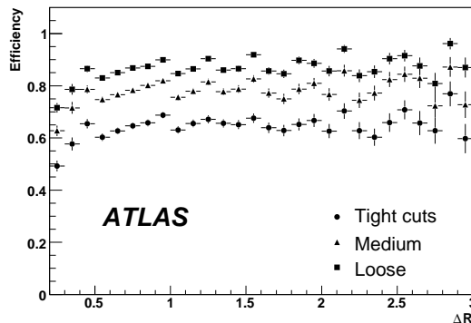
Figure 13: Electron identification efficiency as a function of the distance \Delta R to the closest jet in SUSY events, for electrons with E_T > 17 GeV.
