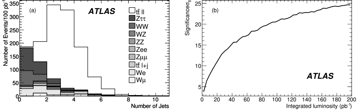
Figure 15: (a) Total composition of the inclusive di-lepton selection versus number of jets. (b) Projected significance from pseudo-experiments for the inclusive template fit versus integrated luminosity including all channels and all systematic uncertainties.
