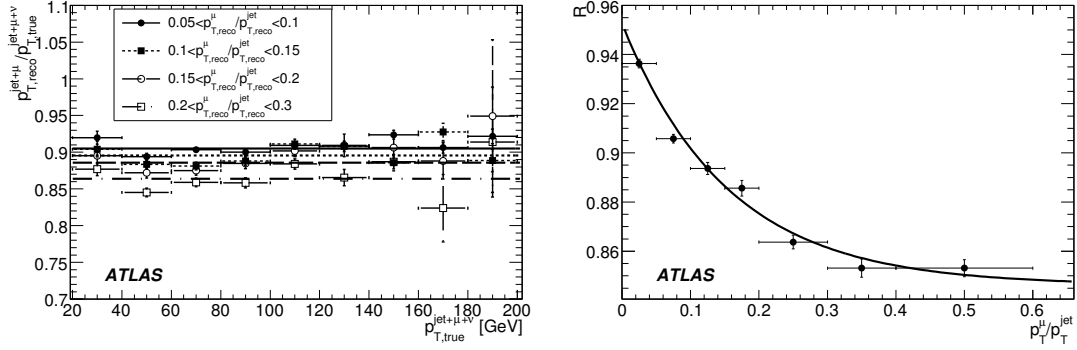
Figure 25: Left: Jet response as a function of jet p_T for semileptonic b jets containing one muon for different values of x (equation 15). Here p_{T, \text{true}}^{\text{jet}+\mu+\nu} refers to the transverse component of the vector addition of the true jet momentum (all interacting particles except muons included), the true muon momentum and the neutrino momentum. Right: Value of the results from straight line fits to the points in the left plot as a function of x . The fit function C(x) = a + b e^{-cx} is also shown.
