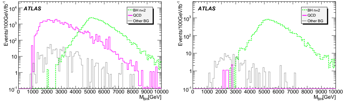
Figure 14: Black hole mass distribution for the signal sample with n = 2 and m > 5 TeV and backgrounds (see Table 7) after multiplicity requirement of at least 4 objects with p_T > 200 GeV (left plot) and an additional requirement of a lepton (electron or muon) with p_T > 200 GeV (right plot).
