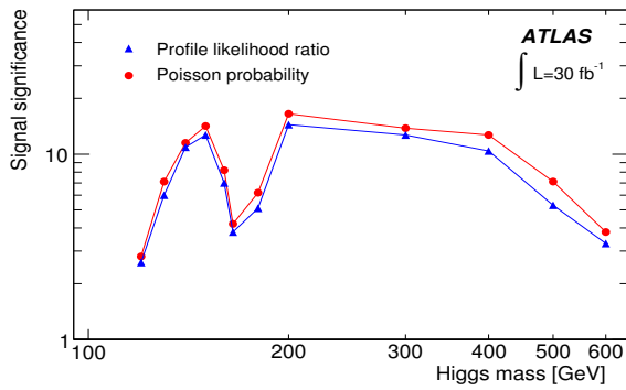
Figure 36: Significance obtained from the profile likelihood ratio, as a function of the Higgs boson mass. The result is compared with the one shown in Section 4 where systematic errors on signal and background have not been included, and the significance has been calculated using Poisson statistics.
