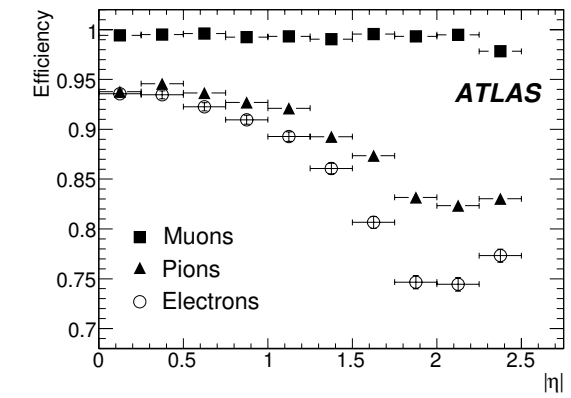
Figure 13: Track reconstruction efficiencies as a function of |\eta| for muons, pions and electrons with p_T = 5 GeV. The inefficiencies for pions and electrons reflect the shape of the amount of material in the inner detector as a function of |\eta| .
