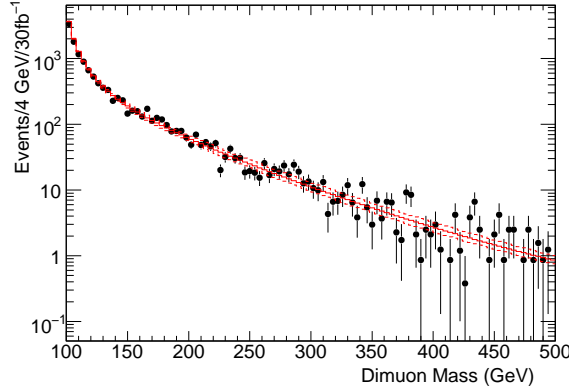
Figure 20: Fit (full line) of the background function f_{bkg} (see Eq. 1) on the background distribution (full circles) resulting from the analysis with at least one b-jet in the final state. The dashed lines represent the shape variations given by the errors on the a_2 and a_3 parameters, from the fit on the e^+e^- data.
