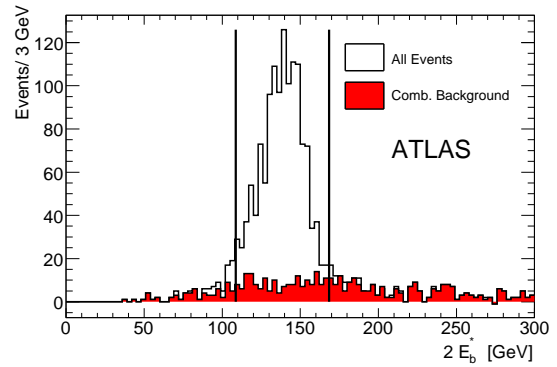
Figure 12: Distribution of X_2 \equiv 2E_b^* for events passing C2, C3, and C4. Vertical lines correspond to the bounds of the C5 cut.
