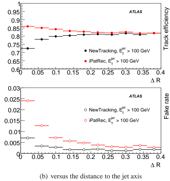
Figure 3: Tracking efficiency (top plots) and fake rate (bottom plots) in t\bar{t} events after the b -tagging quality cuts, for two tracking algorithms: default NewTracking (black symbols) and iPatRec (red symbols).
