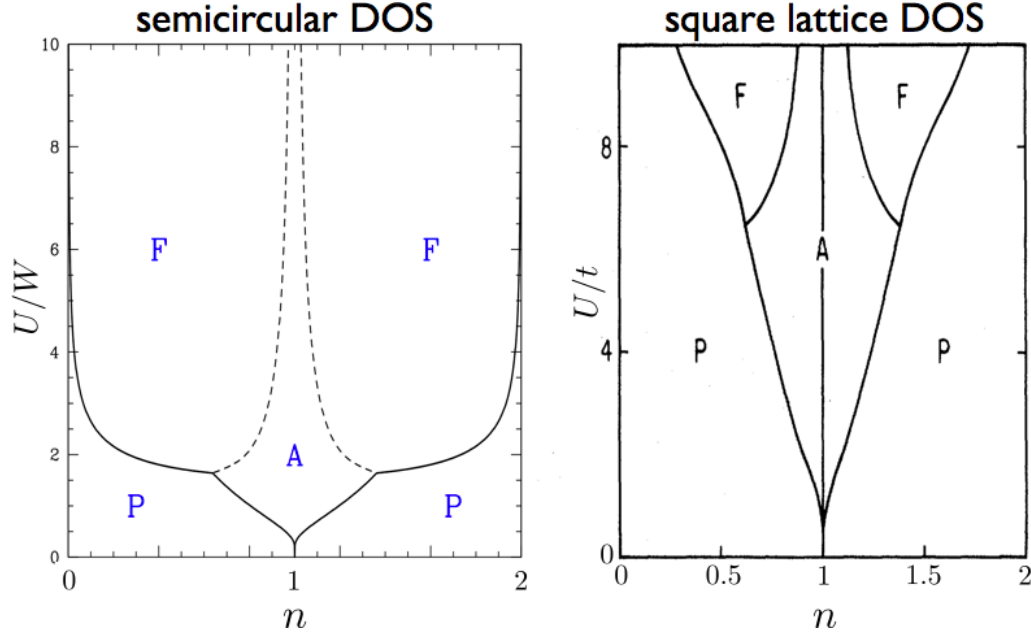
Figure 4.5: Mean field phase diagram of the Hubbard model, including paramagnetic (P), ferromagnetic (F), and antiferromagnetic (A) phases. Left panel: results using a semicircular density of states function of half-bandwidth W . Right panel: results using a two-dimensional square lattice density of states with nearest neighbor hopping t , from J. E. Hirsch, Phys. Rev. B 31 , 4403 (1985). The phase boundary between F and A phases is first order.
