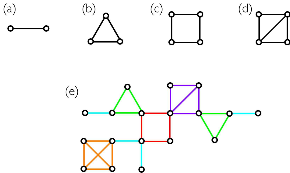
Figure 6.24: Connected versus irreducible clusters. Clusters (a) through (d) are irreducible in that they remain connected if any component site and its connecting links are removed. Cluster (e) is connected, but is reducible . Its integral c_\gamma may be reduced to a product over its irreducible components, each shown in a unique color.
