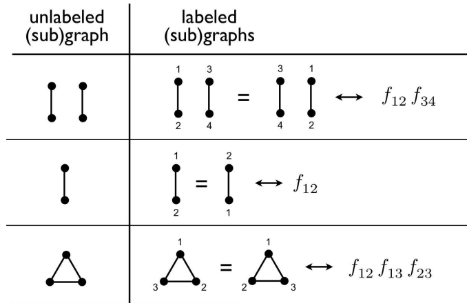
Figure 6.8: Different assignments of labels to vertices may not result in a distinct term in the expansion of the configuration integral.
