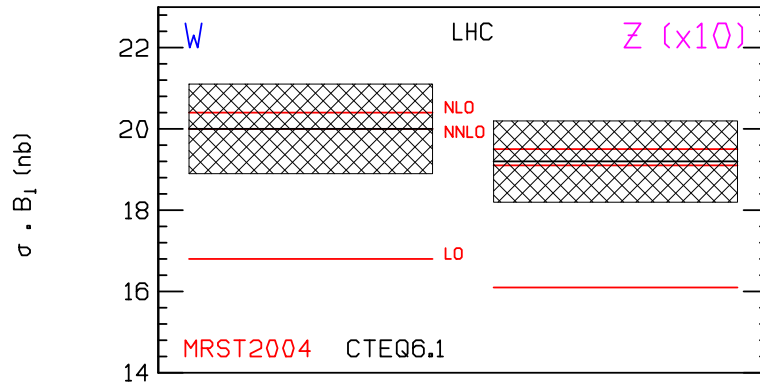
Figure 80. Predicted cross sections for W and Z production at the LHC using MRST2004 and CTEQ6.1 pdfs. The overall pdf uncertainty of the NLO CTEQ6.1 prediction is approximately 5%, consistent with Figure 77.
