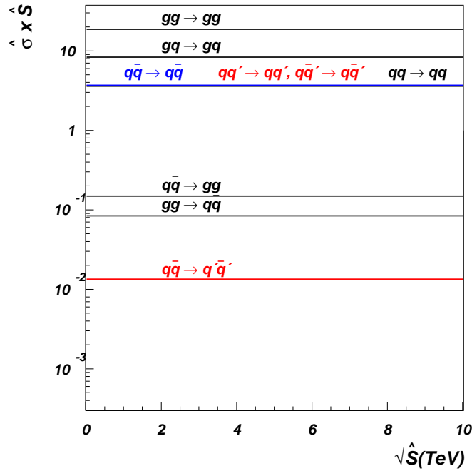
Figure 70. Parton level cross sections ( \hat{\sigma}\hat{\sigma}_{ij} ) for various processes involving massless partons in the final state.
