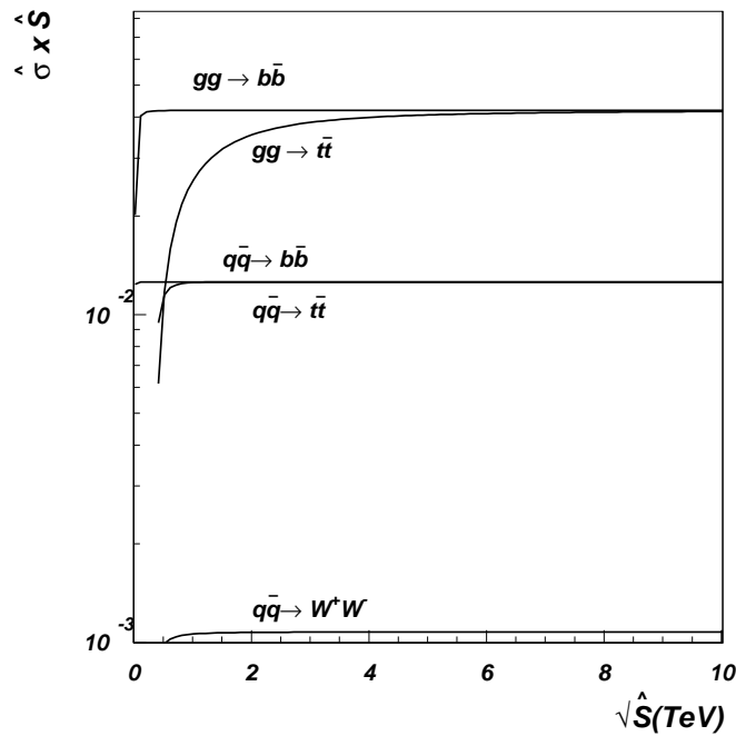
Figure 71. Parton level cross sections ( \hat{\sigma}\hat{\sigma}_{ij} ) for various processes involving massive partons in the final state.
