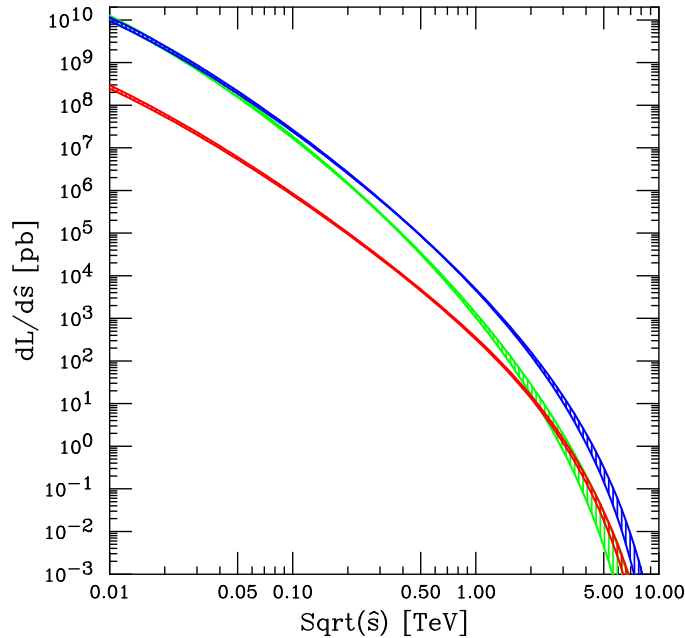
Figure 69. The parton-parton luminosity \left[\frac{dL_{ij}}{d\tau}\right] in picobarns, integrated over y . Green= gg , Blue= \sum_i(gq_i + g\bar{q}_i + q_i g + \bar{q}_i g) , Red= \sum_i(q_i\bar{q}_i + \bar{q}_i q_i) , where the sum runs over the five quark flavours d, u, s, c, b .
