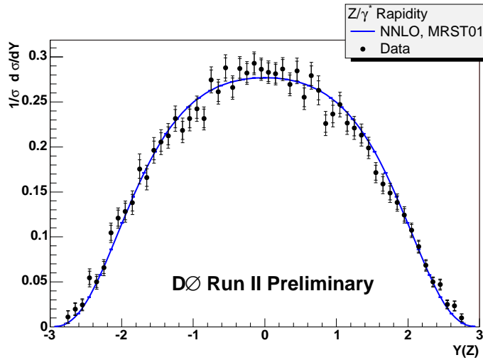
Figure 39. Z rapidity distribution from D0 in Run 2.
