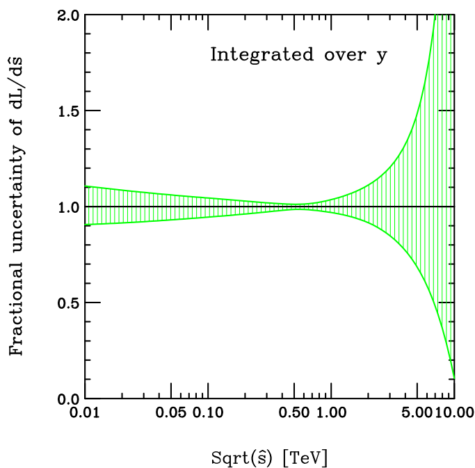
Figure 75. Fractional uncertainty of the gg luminosity integrated over y .
