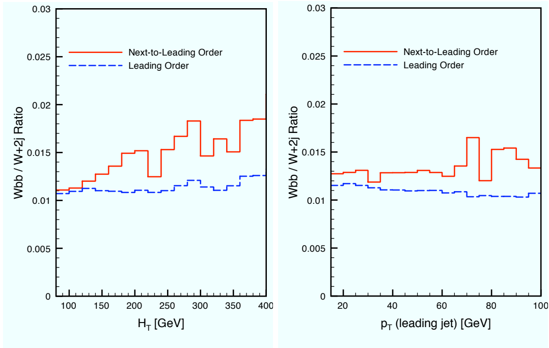
Figure 62. The ratio of the cross sections for Wb\bar{b} and Wjj is plotted at LO and NLO as a function of the variables H_T (left) and the p_T of the leading jet (right). The ratio is observed to have a different slope at NLO than at LO on the left, but a similar slope on the right.
