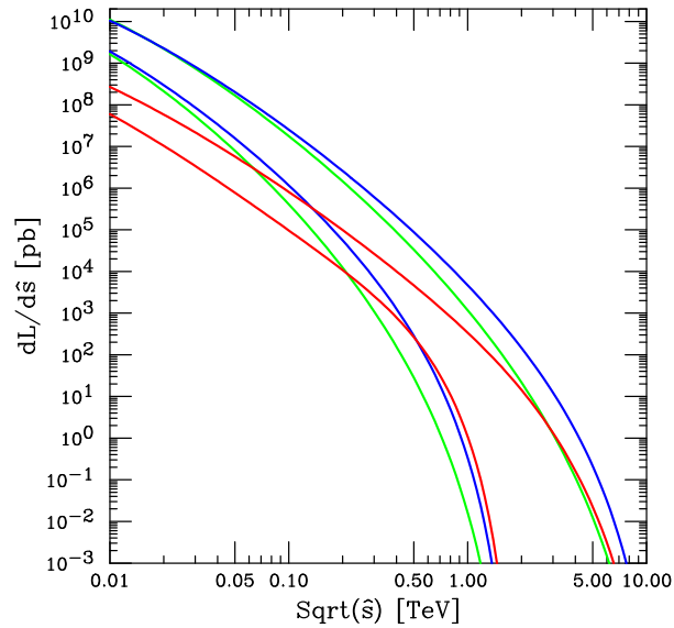
Figure 78. The parton-parton luminosity \left[ \frac{1}{\hat{s}} \frac{dL_{ij}}{d\tau} \right] in pb integrated over y . Green= gg , Blue= \sum_i (q_i q_i + g \bar{q}_i + q_i g + \bar{q}_i g) , Red= \sum_i (q_i \bar{q}_i + \bar{q}_i q_i) , where the sum runs over the five quark flavours d, u, s, c, b . The top family of curves are for the LHC and the bottom for the Tevatron.
