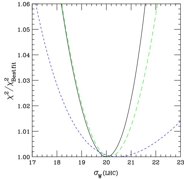
Figure 81. Predicted total cross section of W^+ + W^- production at the LHC for the fits obtained in the CTEQ stability study, compared to the MRST results. The overall pdf uncertainty of the prediction is \sim 5\% , as observed in Figure 77.
