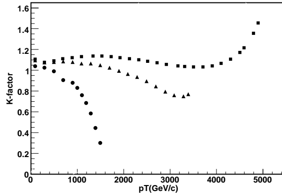
Figure 106. The ratios of the NLO to LO jet cross section predictions for the LHC using the CTEQ6.1 pdfs for the three different rapidity regions (0–1 (squares), 1–2 (triangles), 2–3 (circles)).
