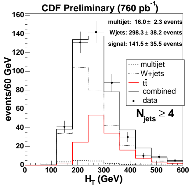
Figure 63. The H_T distribution in W + \geq 4 jet events at CDF, along with the fitted components for t\bar{t} production and backgrounds from W + jets and multijet events.
