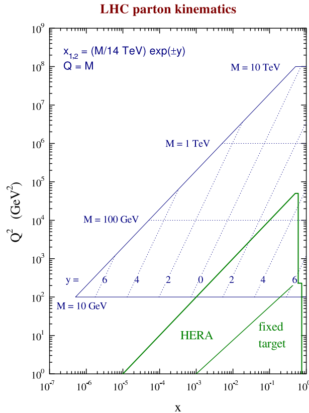
Figure 3. Graphical representation of the relationship between parton ( x, Q^2 ) variables and the kinematic variables corresponding to a final state of mass M produced with rapidity y at the LHC collider with \sqrt{s} = 14 TeV.
