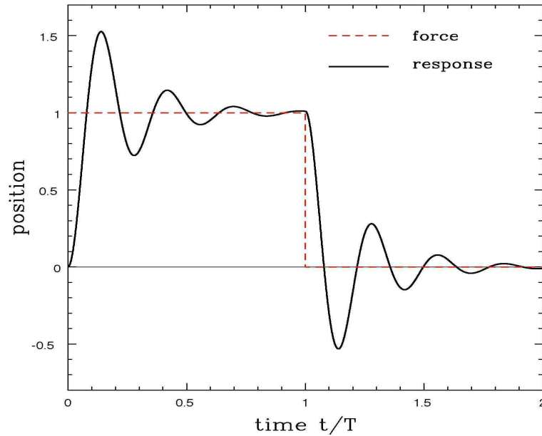
Figure 4.6: Response of an underdamped oscillator to a pulse force.
