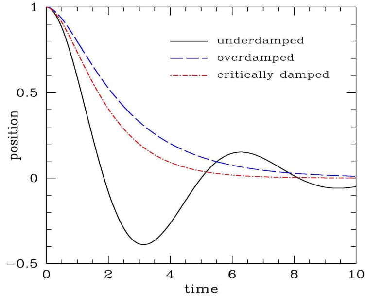
Figure 4.1: Three classifications of damped harmonic motion. The initial conditions are x(0) = 1 , \dot{x}(0) = 0 .
