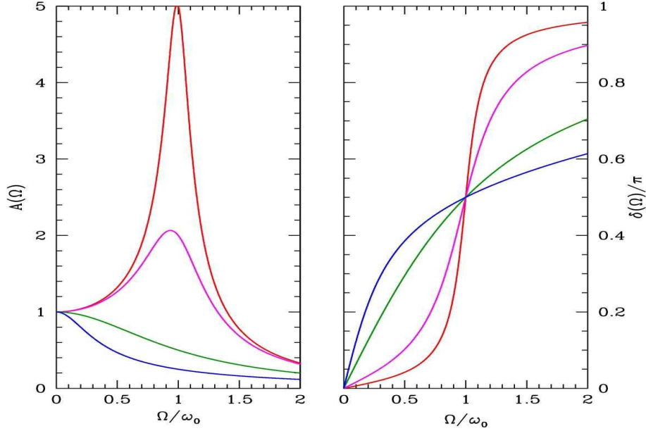
Figure 4.2: Amplitude and phase shift versus oscillator frequency (units of \omega_0 ) for \beta/\omega_0 values of 0.1 (red), 0.25 (magenta), 1.0 (green), and 2.0 (blue).
