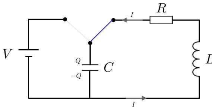
Figure 4.3: An R - L - C circuit which behaves as a damped harmonic oscillator.
