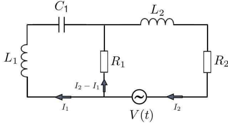
Figure 4.4: A driven L - C - R circuit, with V(t) = V_0 \cos(\omega t) .
