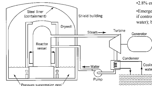
Figure 6.3 A diagram of a boiling water reactor power plant. Steam is produced in the reactor vessel and flows at high pressure to the turbine. After the steam is condensed to water at the low-pressure side of the turbine, the water is recirculated through a pump to the reactor core. The components of the reactor containment building are discussed in the text. Source: A. V. Nero, Jr., A Guidebook to Nuclear Reactors . Berkeley: University of California Press, 1979
