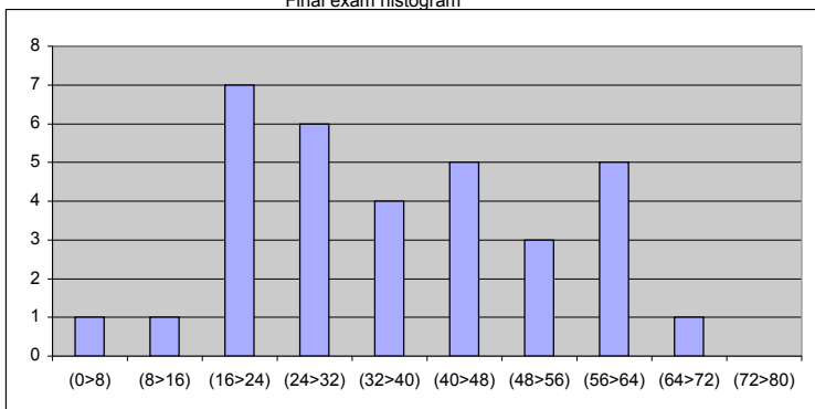
Final exam histogram
