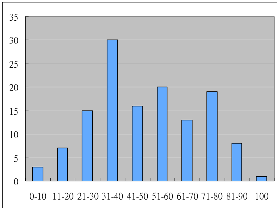
Curriculum Histograms
